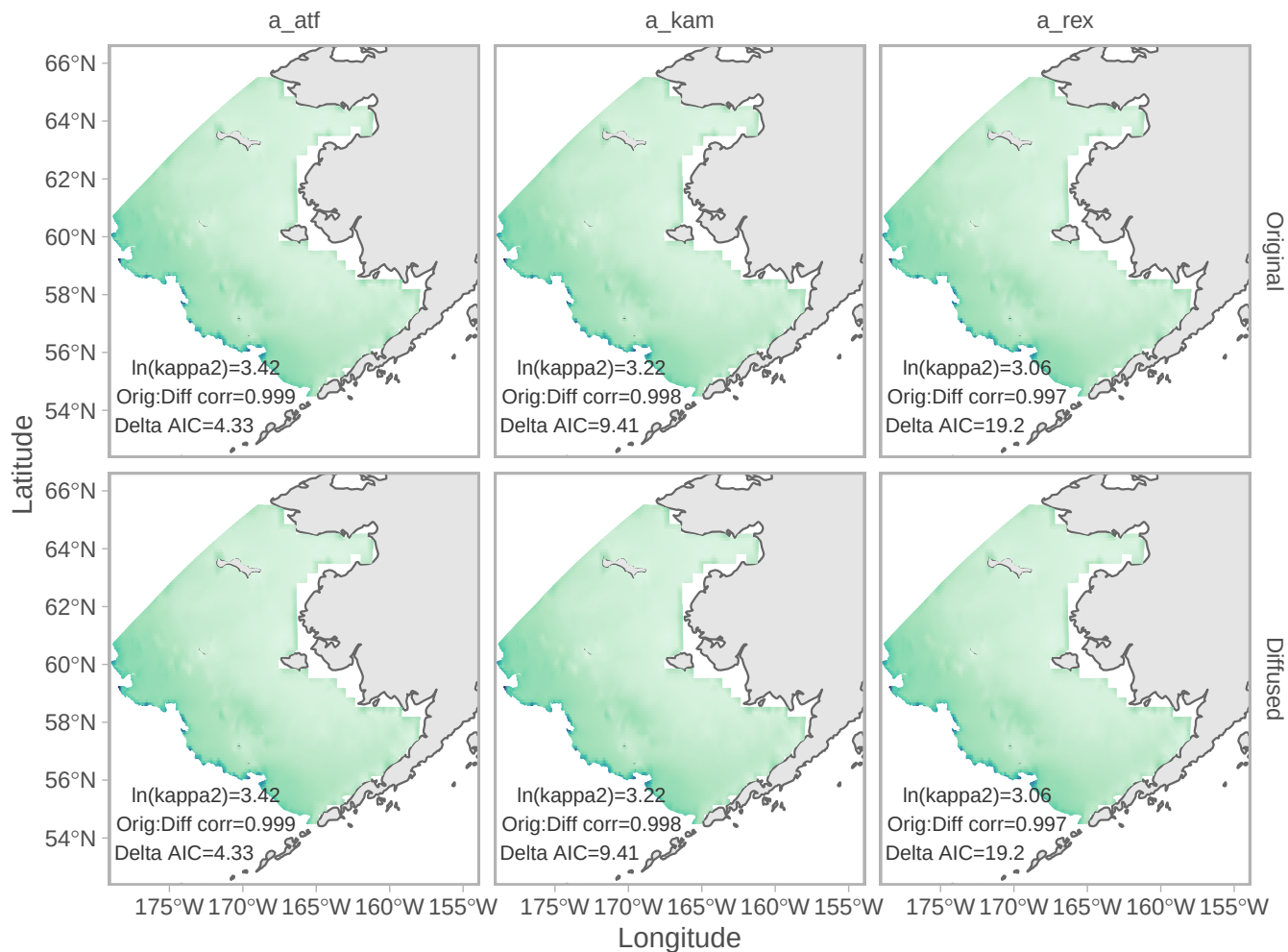
Species with high correlation and high delta AIC
