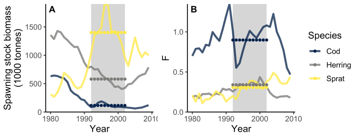
267 268 Figure S4. Time-series of spawning stock biomass (SSB) (A) and fishing mortality (B) from 269 stock assessment model estimates (ICES 2013, 2015). Grey background shows calibration 270 period, dotted horizontal lines show the mean of each time series in the calibration time period.
