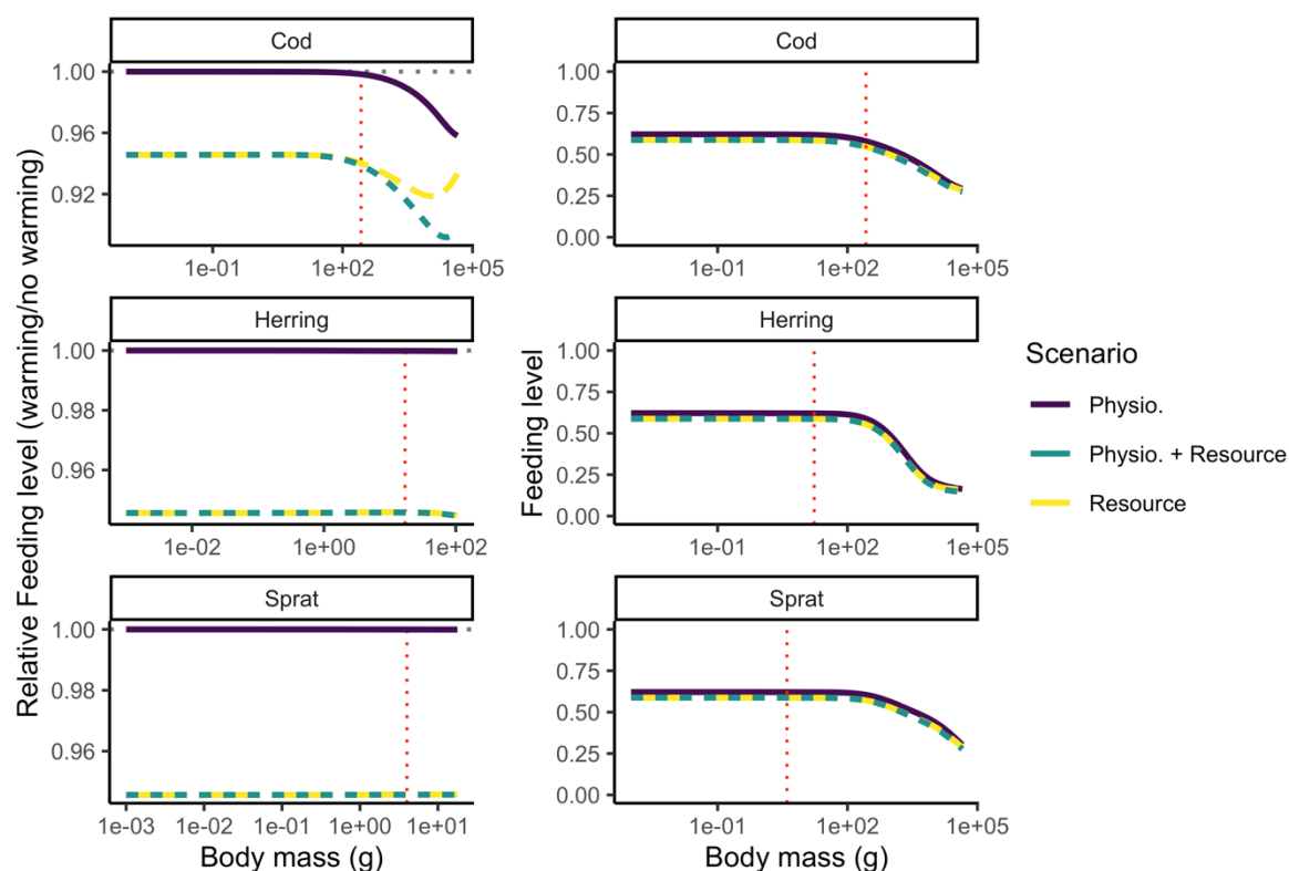
Figure S13. Feeding levels from model projections to 2050 assuming warming according to RCP 8.5 while keeping fishing mortality at average F_{MSY} levels (as estimated at T_{ref} ). Left column shows feeding levels relative to a non-warming simulation (i.e., dashed horizontal grey line) and right column shows absolute feeding level. Activation energies are the means of their respective distributions (no uncertainty).
