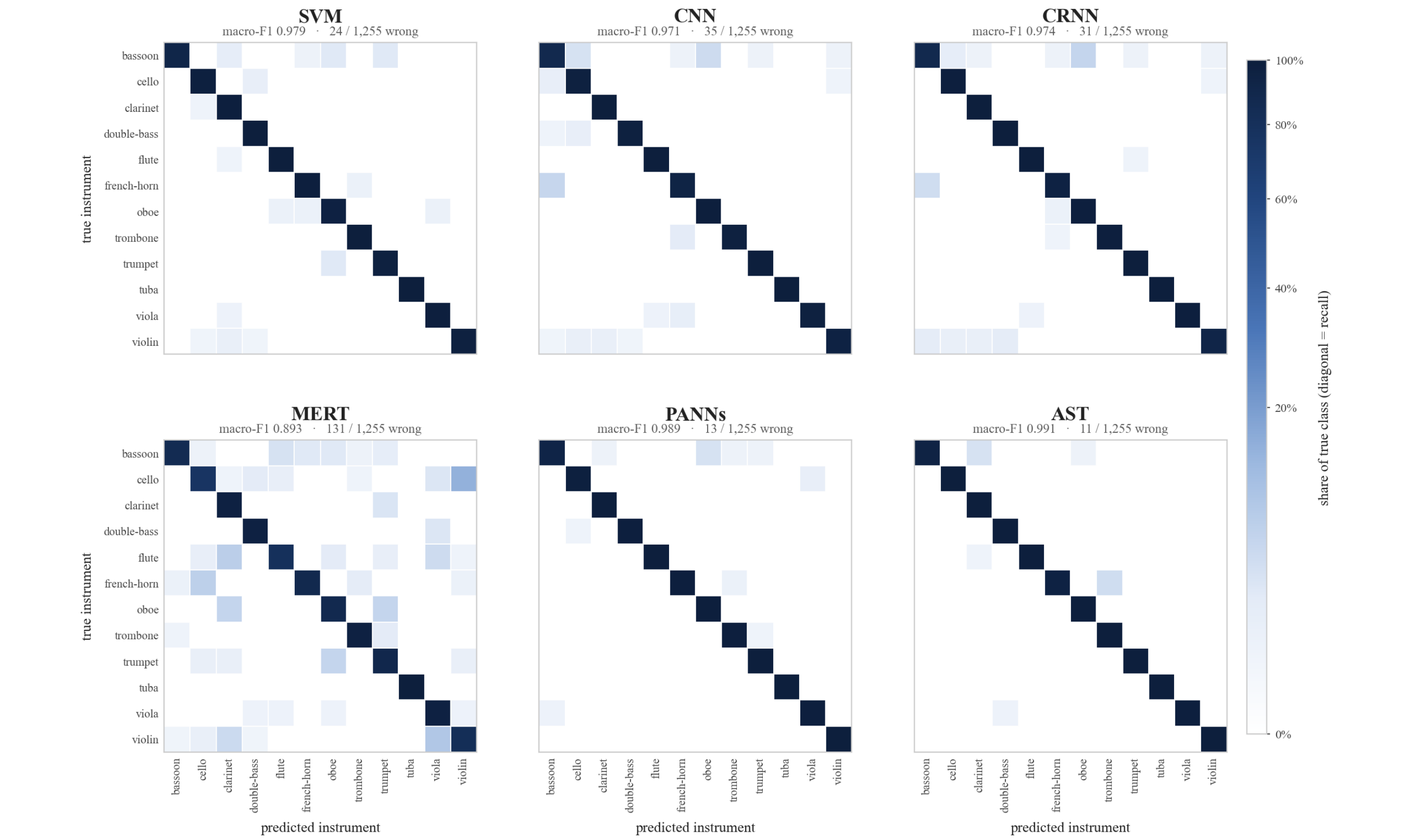
Figure 7. Clean-audio confusion for all six models, row-normalised: the diagonal is per-class recall, off-diagonal cells are the share of a true instrument sent elsewhere, on one colour scale across panels. Panel titles give clean macro-F1 and total misclassified windows.
