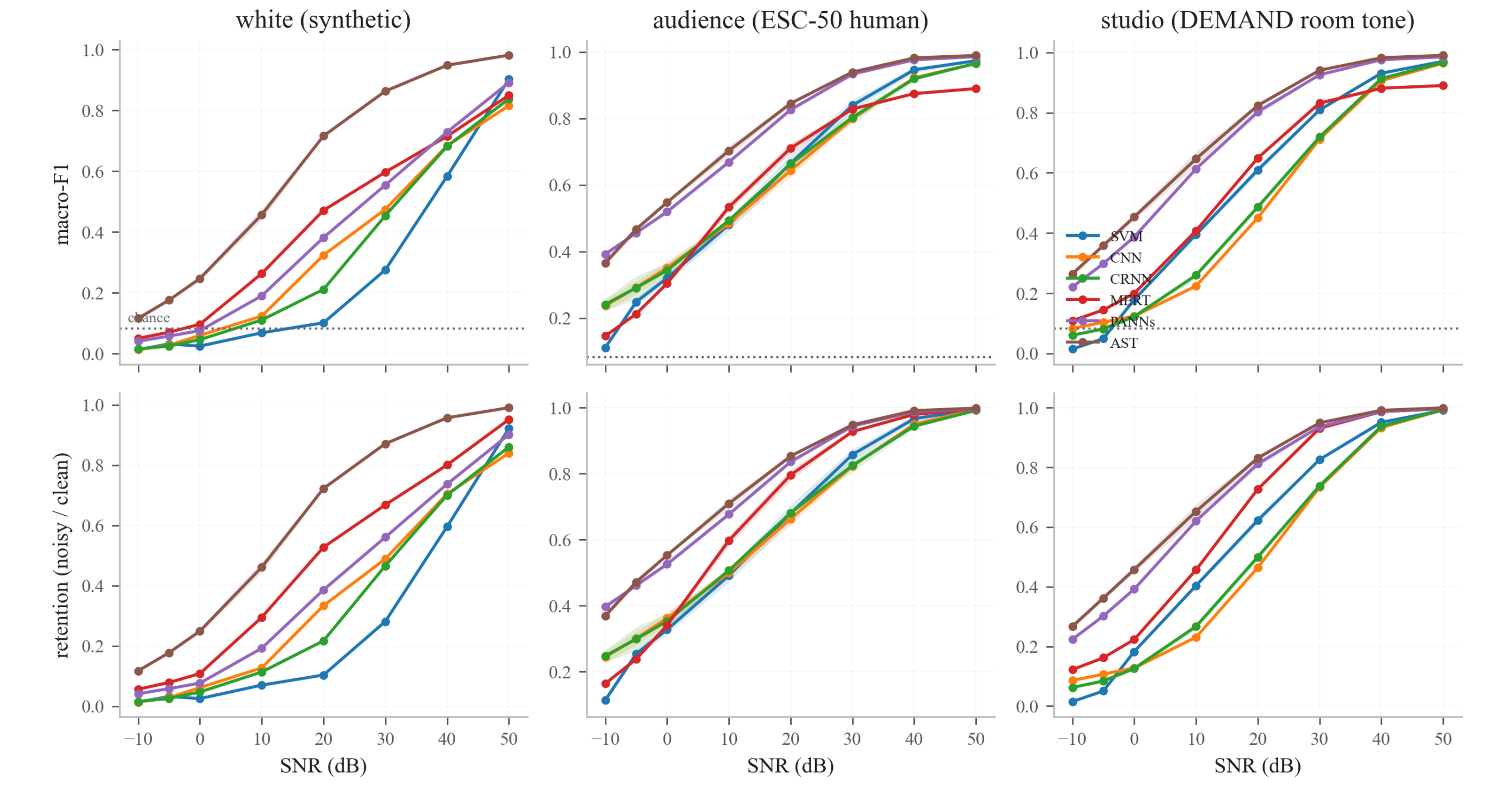
Figure 6. Robustness curves for all 6 models across 3 noise types (columns): macro-F1 (top row) and retention relative to clean score (bottom row), versus SNR from 50 to −10 dB. Shaded band is the spread across two noise draws; dotted line is 12-class chance (0.083).
