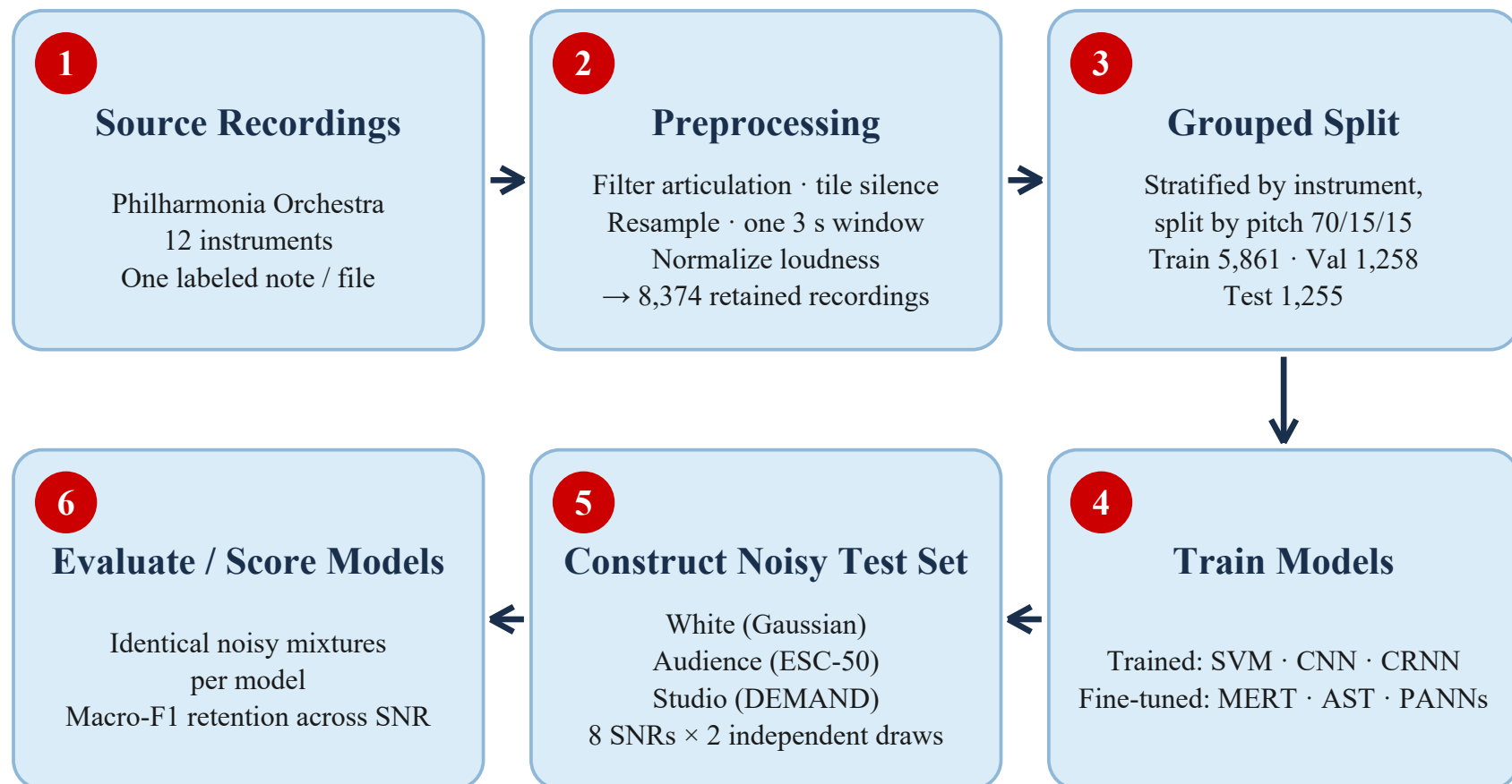
Fig.2 Methods pipeline
