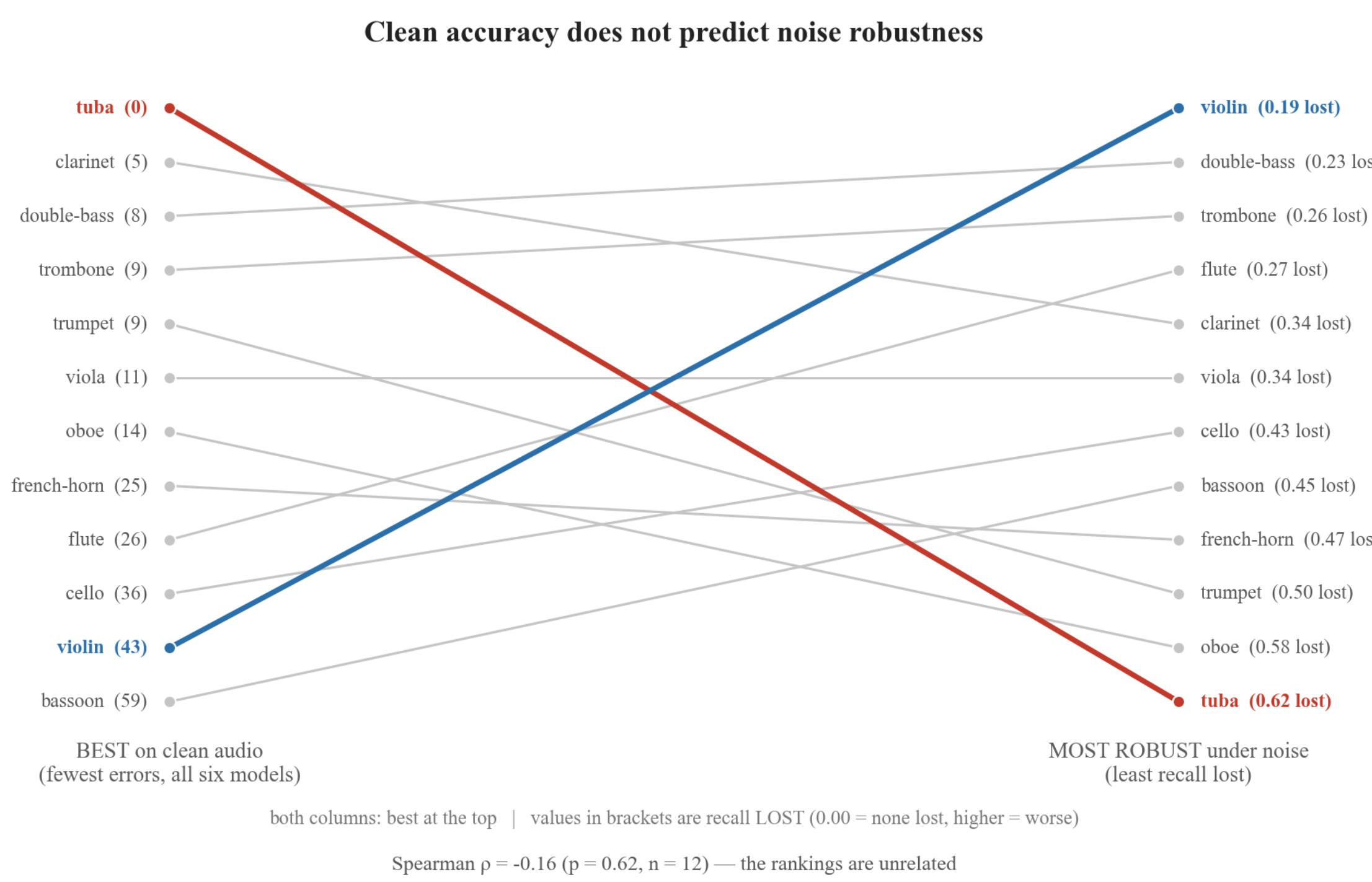
Figure 8. Instruments ranked by clean accuracy (left) and noise robustness (right), best at top. The rankings are unrelated (Spearman \rho = -0.16 , p = 0.62 ). Tuba is classified perfectly by all six models but loses the most recall under noise (0.62); violin is 43 clean errors yet the most robust (0.19 lost).
