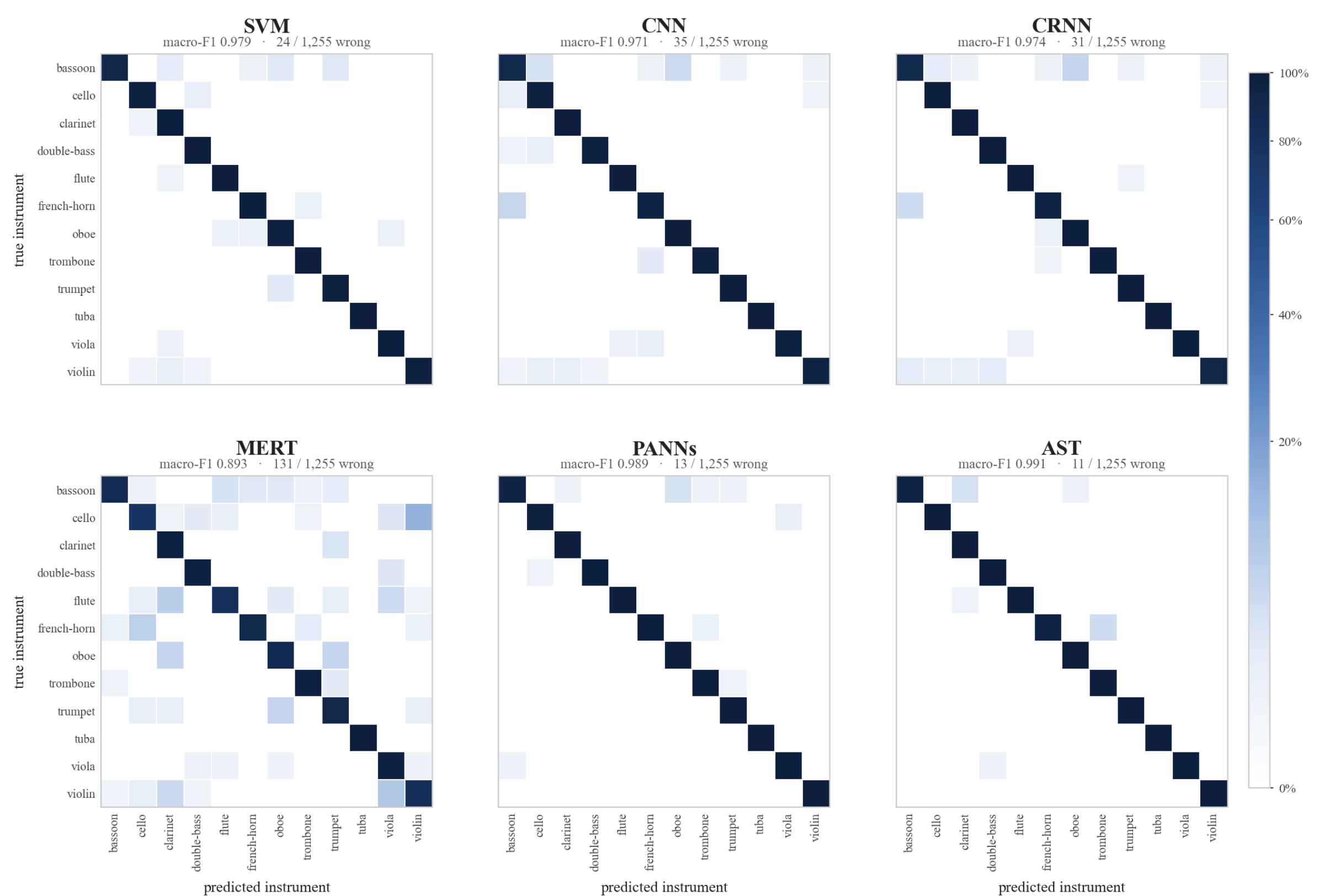
Figure 7. Clean-audio confusion for all six models, row-normalized: the diagonal is per-class recall, off-diagonal cells are the share of a true instrument sent elsewhere, on one colour scale across panels. Panel titles give clean macro-F1 and total misclassified windows.
