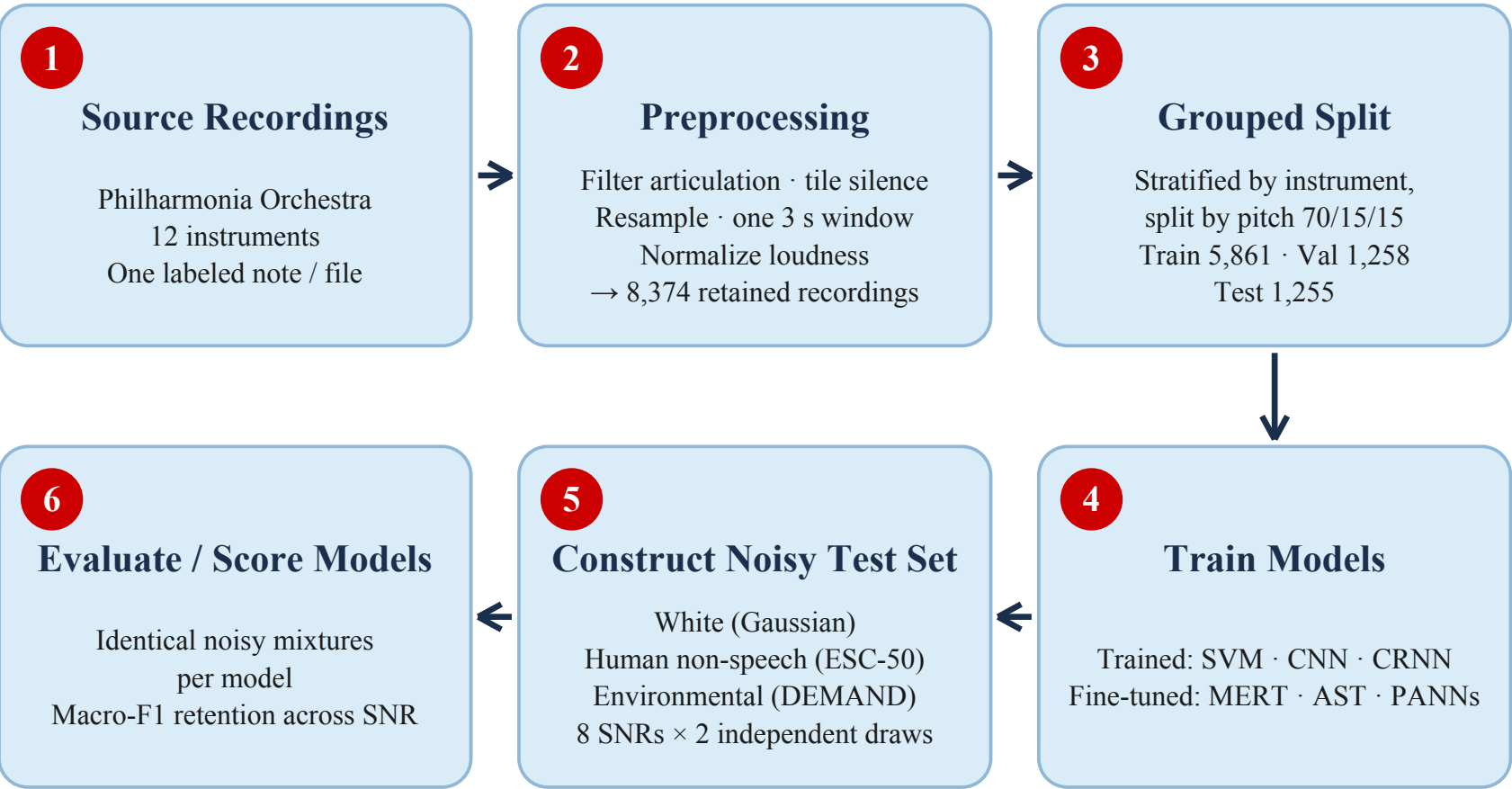
Fig.2 Methods pipeline
