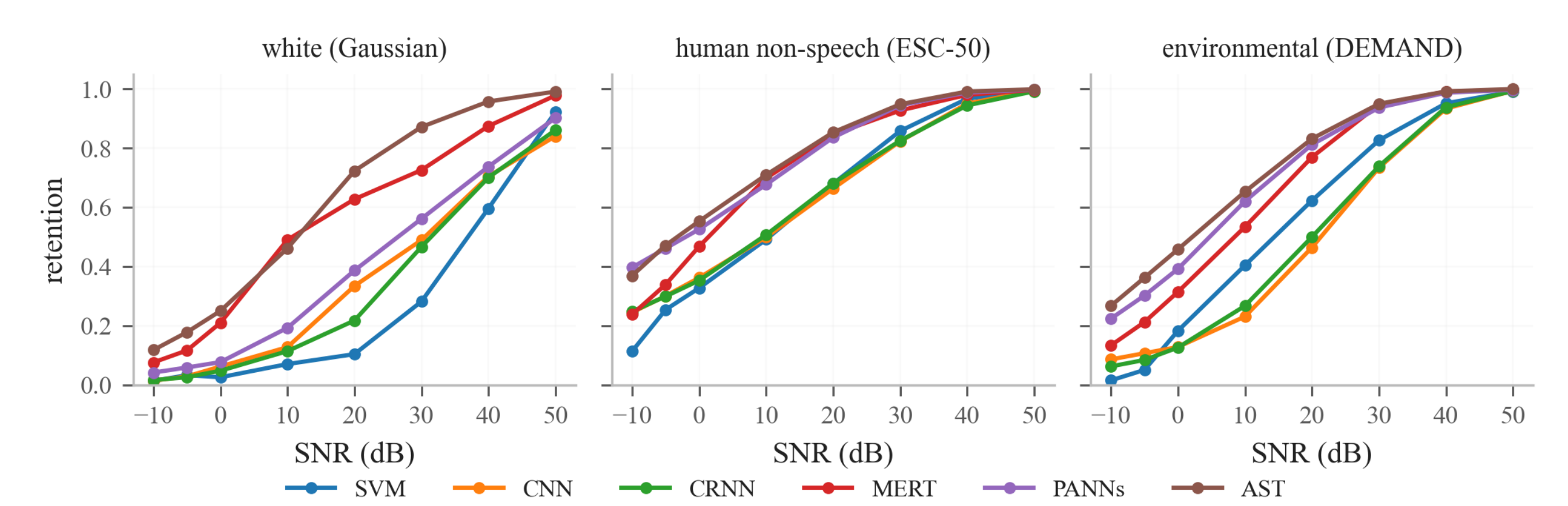
Figure 6. Retention relative to clean macro-F1 versus SNR for all six models and three noise categories. Each point averages two noise realizations.
