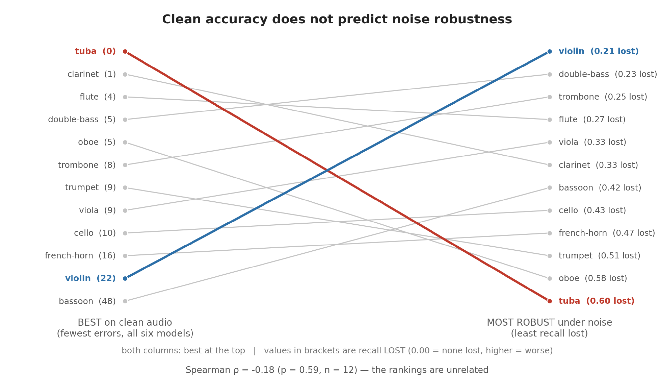
Figure 8. Instruments ranked by clean errors (left) and mean recall-loss AUC under noise (right), best at top. The rankings were unrelated (Spearman \rho = -0.18 , p = 0.59 ). Tuba had no clean errors but the greatest recall loss (0.60); violin had 22 clean errors but the smallest loss (0.21).
