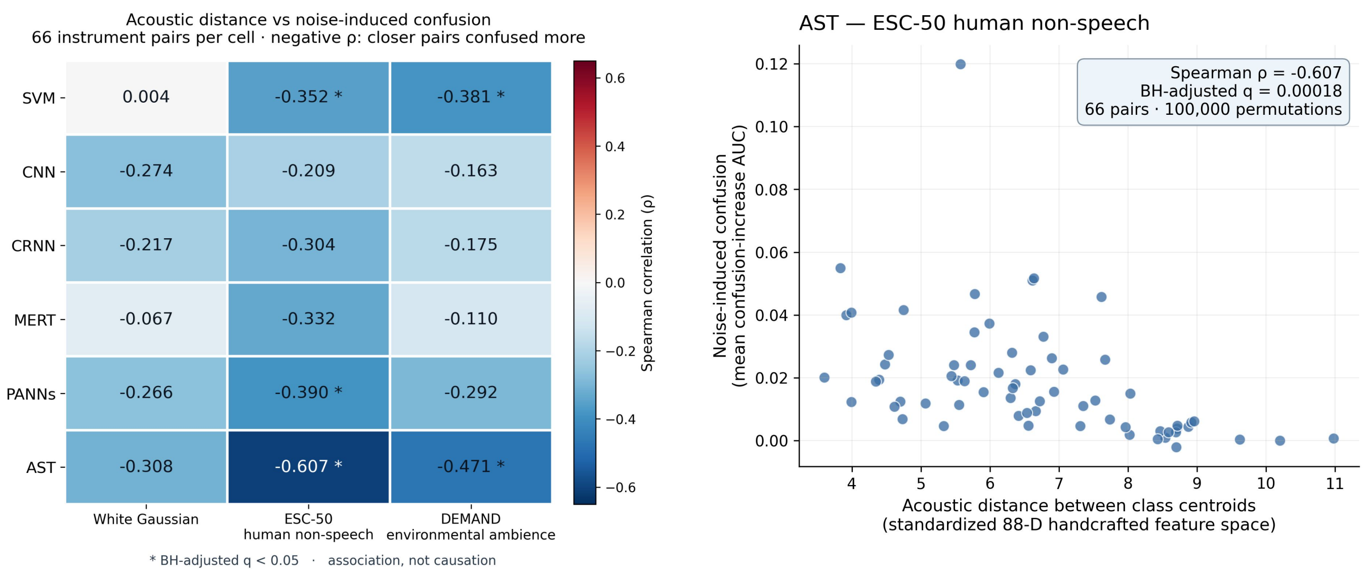
Figure 9b. Illustrative AST x ESC-50 human non-speech relationship across 66 instrument pairs
