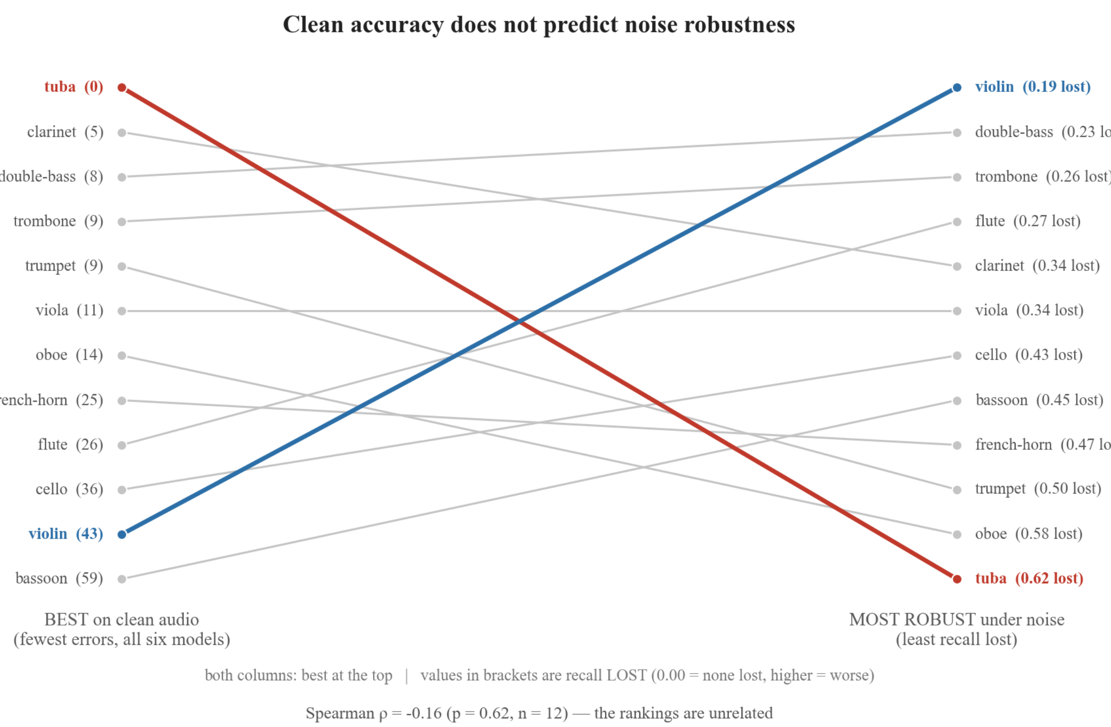
Figure 8. Instruments ranked by clean accuracy (left) and noise robustness (right), best at top. The rankings are unrelated (Spearman \rho = -0.16 , p = 0.62 ). Tuba is classified perfectly by all six models but loses the most recall under noise (0.62); violin is 43 clean errors yet the most robust (0.19 lost).
