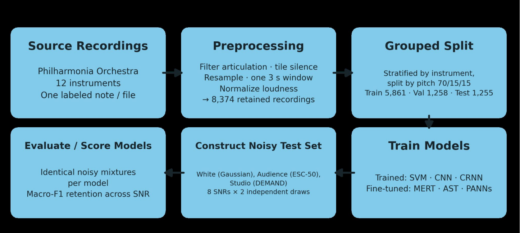
Fig.2 Methods pipeline summary, beginning to end
