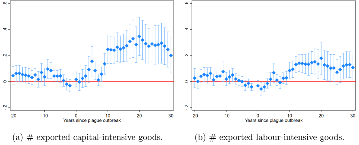
Figure 22: Extensive margin expansion, by factor intensity.
