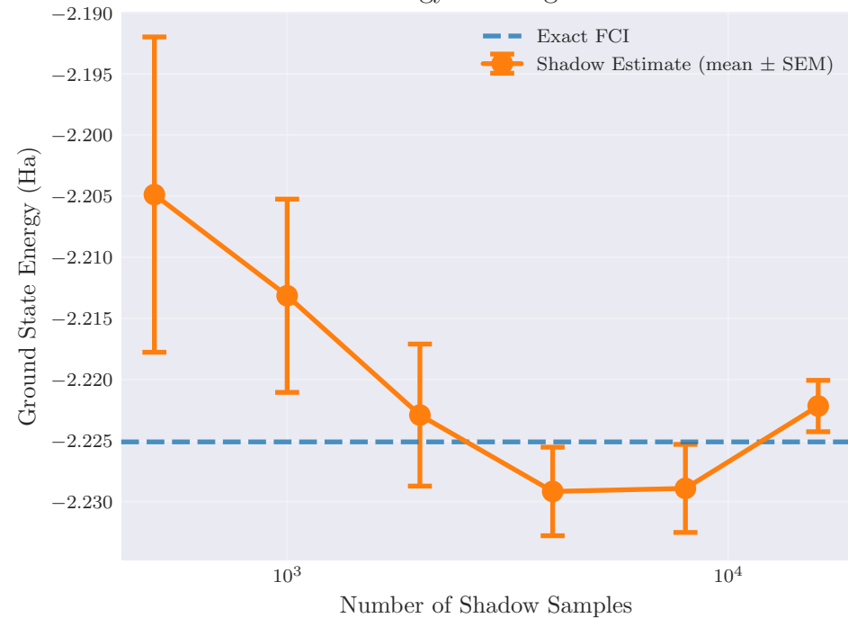
Energy Convergence
