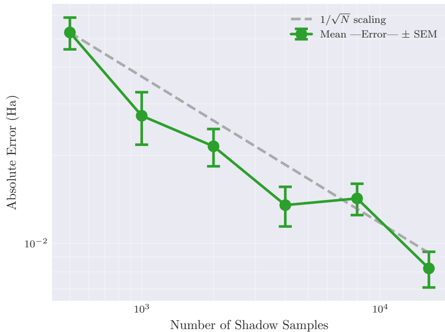
Error Scaling
