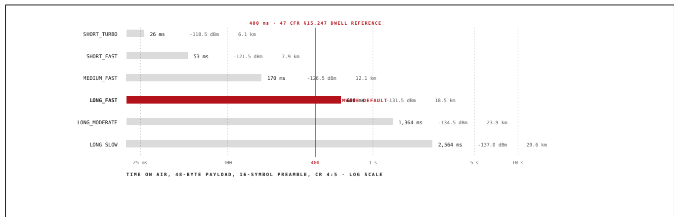
FIGURE 2: TIME ON AIR AND THE DWELL BUDGET
