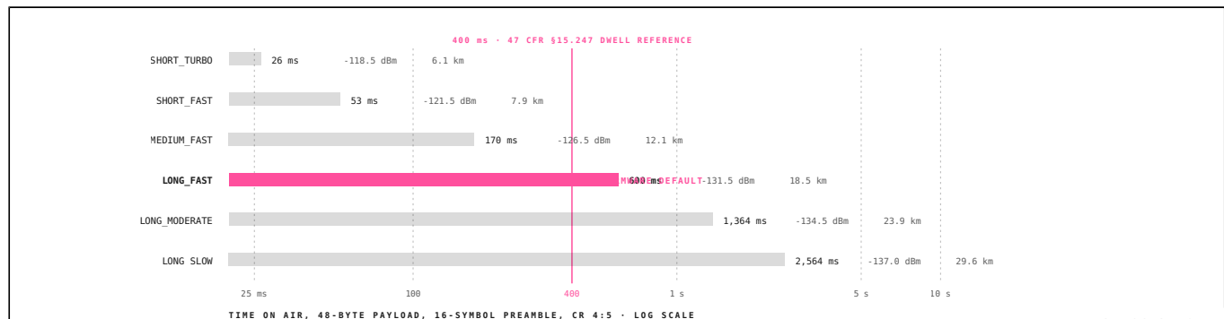
FIGURE 2: TIME ON AIR AND THE DWELL BUDGET
