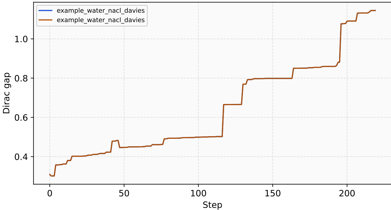
Comparison: Dirac gap
