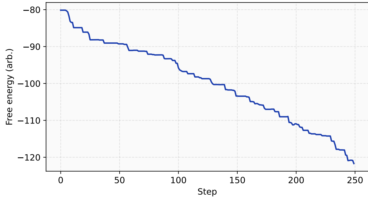
Energy relaxation
