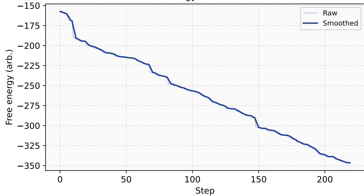
Energy relaxation
