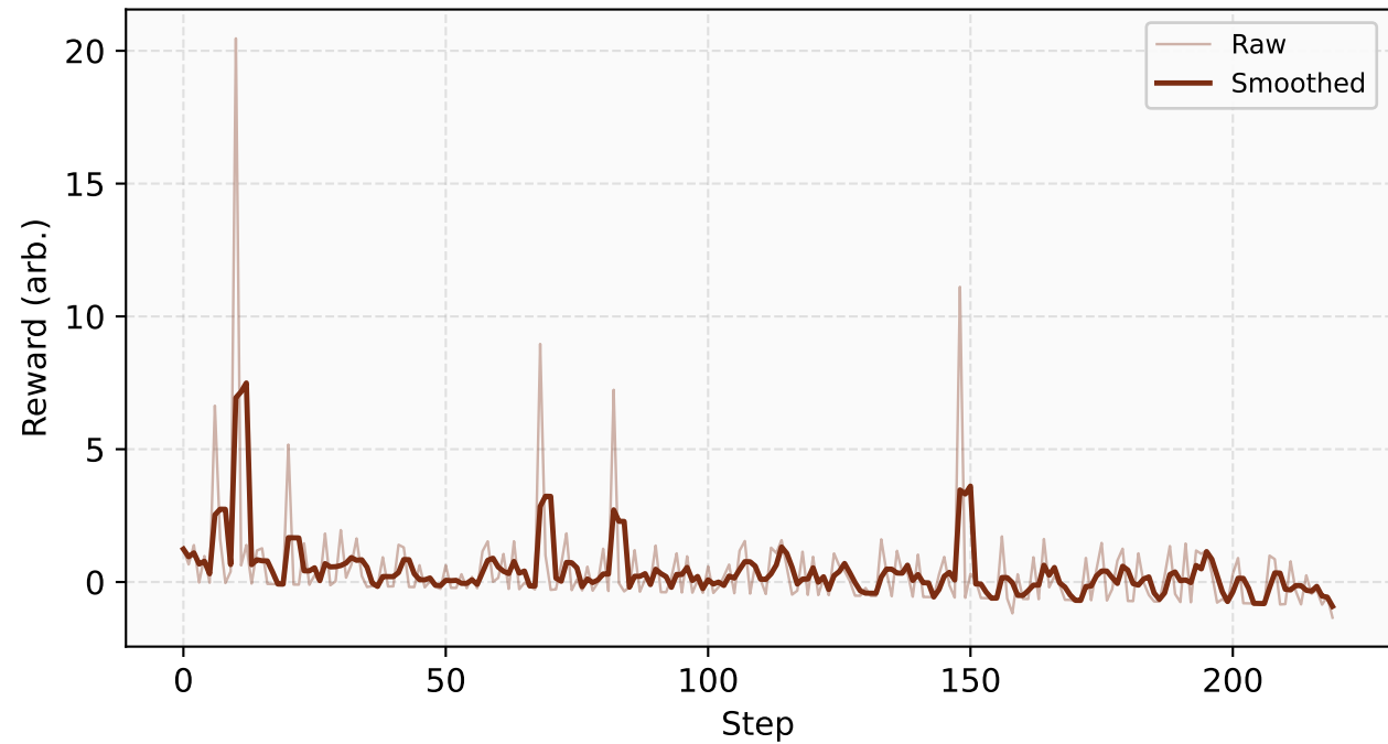
Reward trajectory
