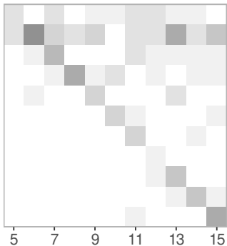
Qwen2.5-7B
