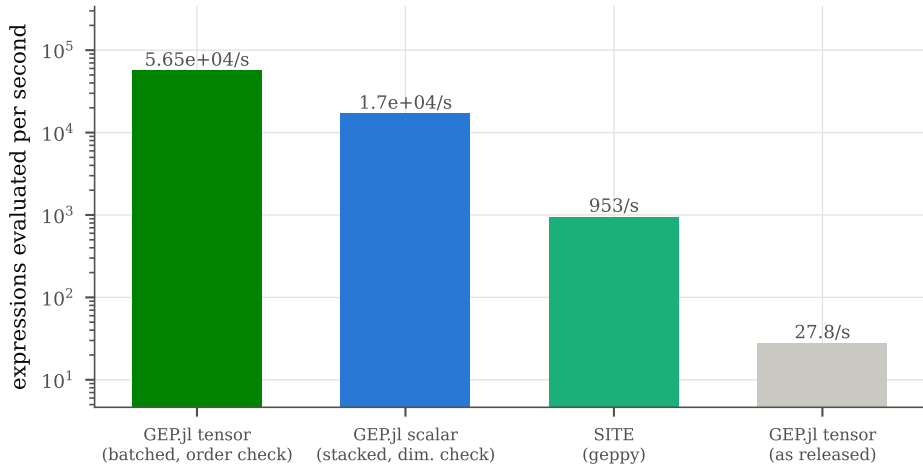
Evaluation throughput on the 150-sample Maxwell case
