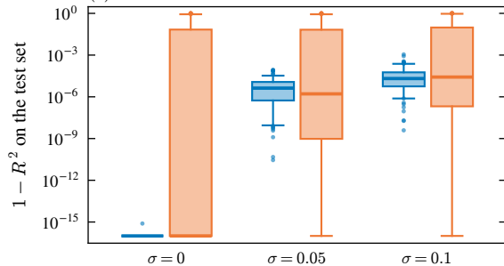
(c) Test error
