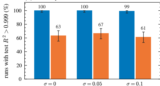
(b) Accuracy solution rate
