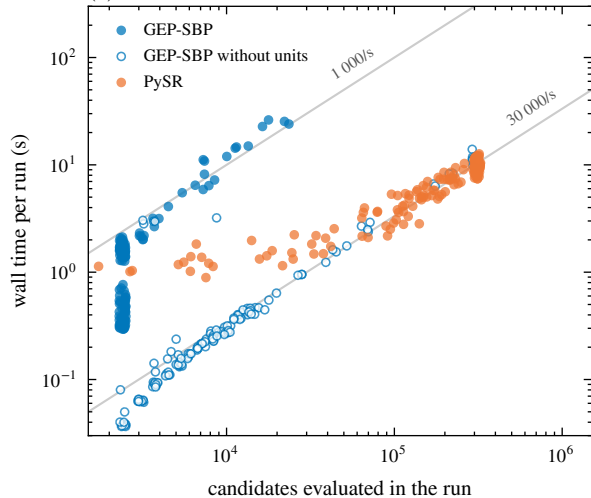
(a) Candidates and time, \sigma = 0
