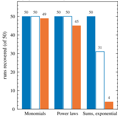
(b) Symbolic recovery, \sigma = 0
