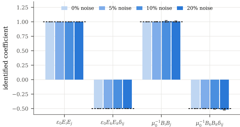
Recovered coefficients, scalar path with the dimensional check (dashed: truth)
