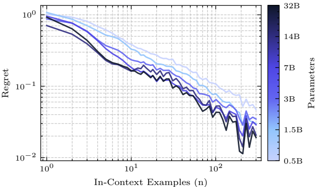
In-Context Learning Regret for H(Y | X) = 0.26
