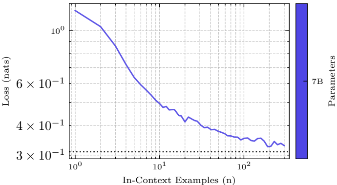
In-Context Learning Loss for H(Y | X) = 0.31
