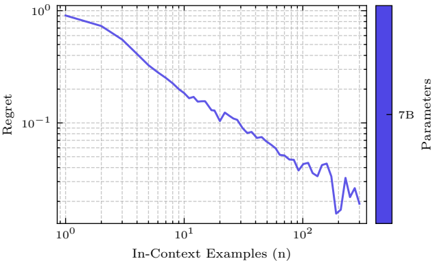
In-Context Learning Regret for H(Y | X) = 0.31
