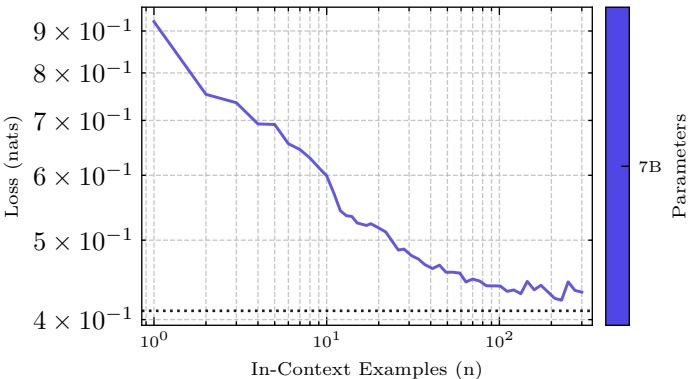
In-Context Learning Loss for H(Y | X) = 0.41
