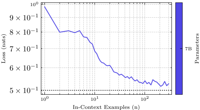
In-Context Learning Loss for H(Y | X) = 0.50
