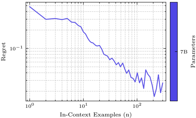
In-Context Learning Regret for H(Y | X) = 0.50
