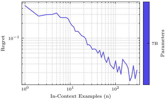
In-Context Learning Regret for H(Y | X) = 0.55
