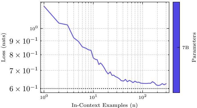
In-Context Learning Loss for H(Y | X) = 0.60
