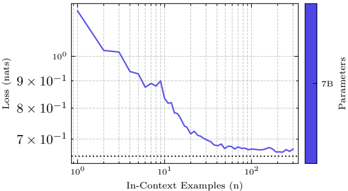
In-Context Learning Loss for H(Y | X) = 0.65
