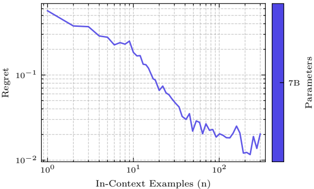
In-Context Learning Regret for H(Y | X) = 0.65
