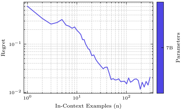
In-Context Learning Regret for H(Y | X) = 0.69
