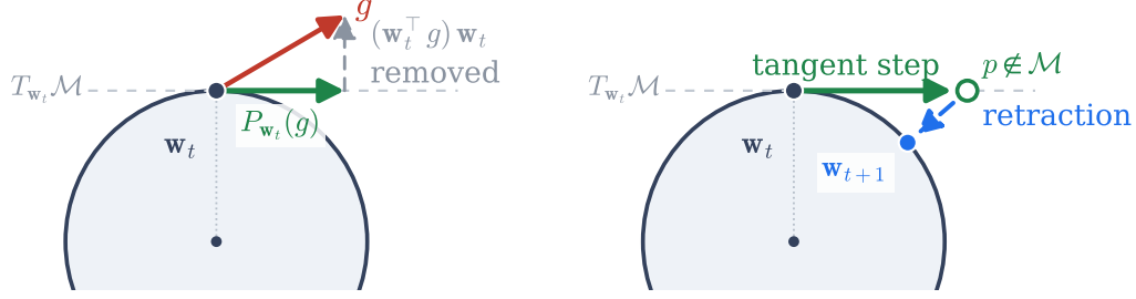
(a) project the gradient onto T_{\mathbf{w}_t}\mathcal{M} (b) step, then retract back onto \mathcal{M}
