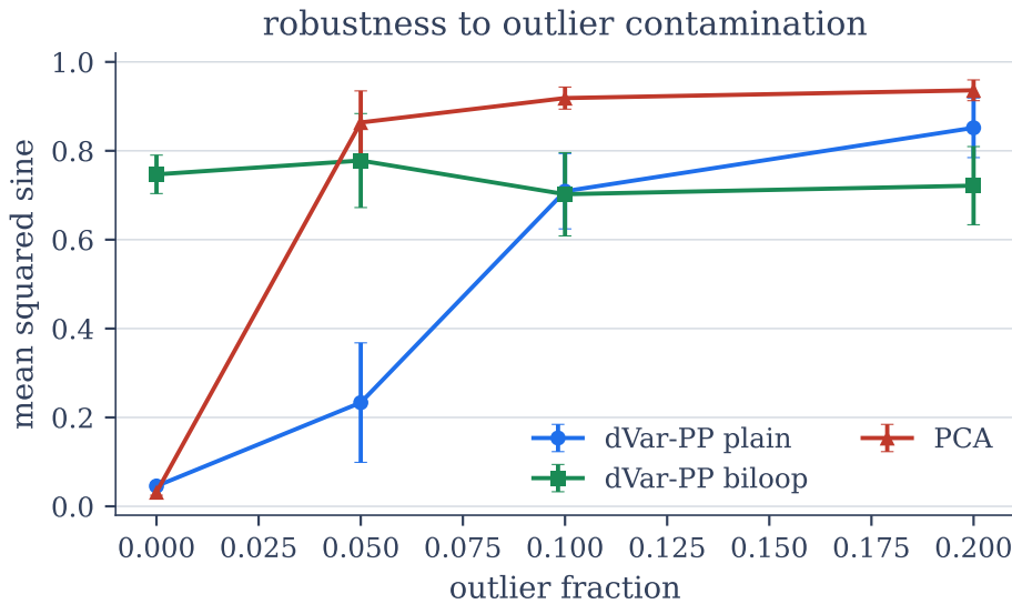
Figure 5.2: Mean squared sine against outlier fraction for plain dVar-PP, biloop dVar-PP and PCA. At 5% contamination the plain index deteriorates less than PCA. The biloop variant starts far worse on clean data and is the flattest of the three under heavy contamination, where no method recovers the subspace.
