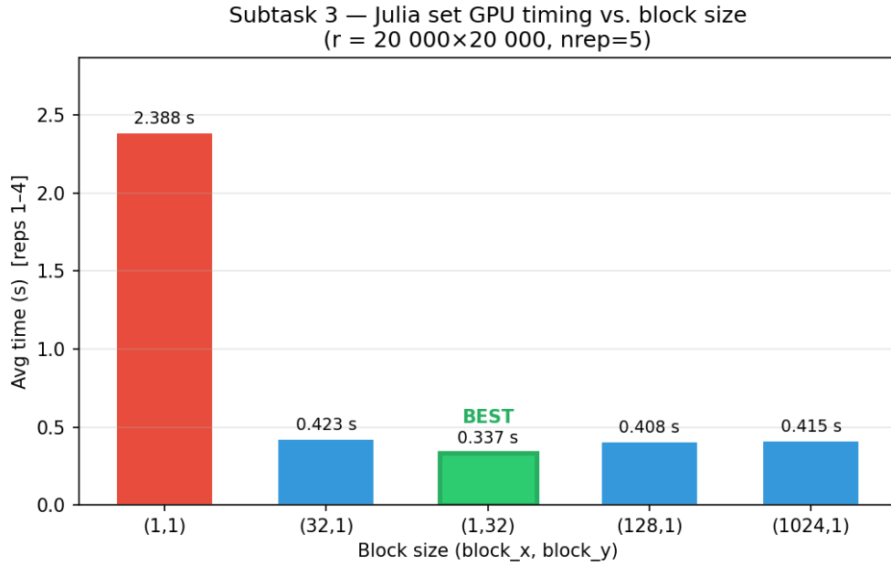
Figure 2: Average steady-state GPU time per block size ( r = 20\,000 \times 20\,000 , \text{nrep} = 5 , reps 1–4). Best configuration (block 1 \times 32 ) highlighted in green.
