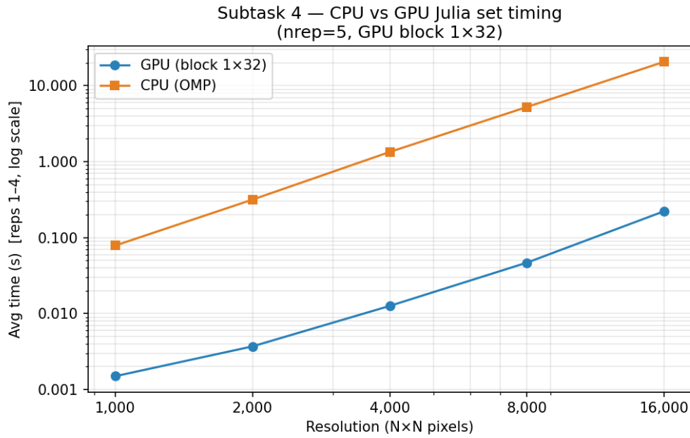
Figure 3: CPU vs. GPU average steady-state time vs. resolution (log–log scale, nrep = 5, reps 1–4). GPU uses best block (1×32); CPU uses OMP_NUM_THREADS=32. No crossover was detected in the measured resolution range.
