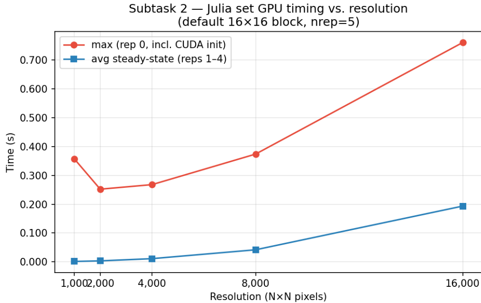
Figure 1: GPU kernel time vs. resolution (default 16 \times 16 block size, nrep = 5 ). Red : maximum time across 5 reps (rep 0, includes CUDA context initialisation). Blue : average steady-state time (reps 1–4).
