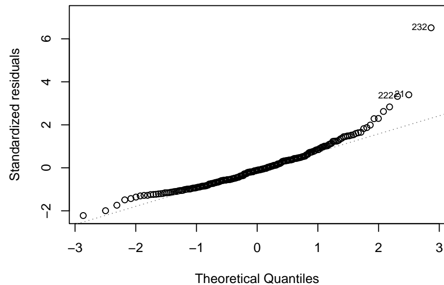
Q-Q Residuals
