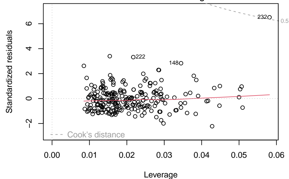
Residuals vs Leverage
