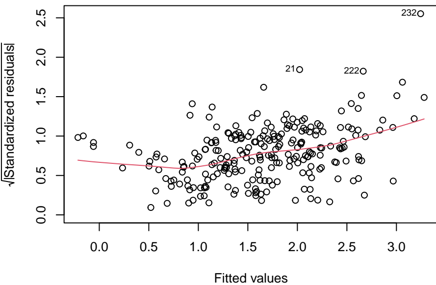
Scale-Location
