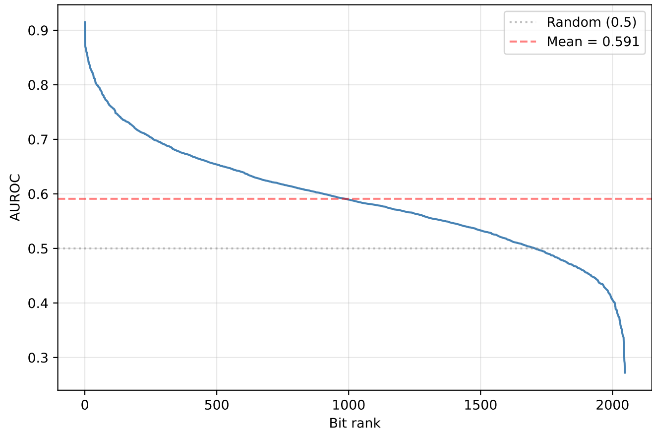
(b) Per-bit AUROC (ranked)
