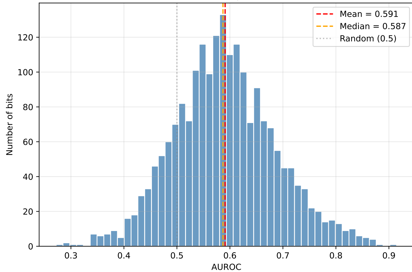
(a) Distribution of per-bit AUROC
