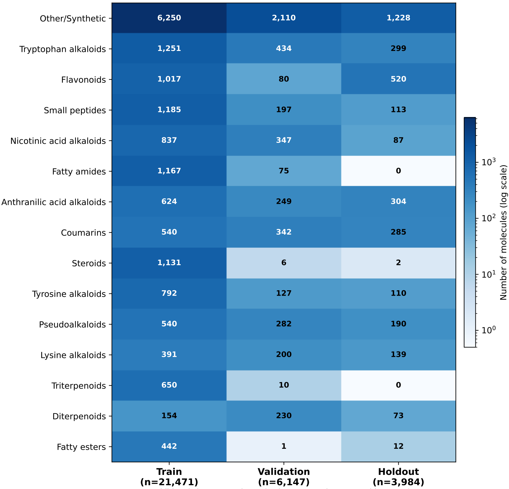
Distribution of Molecular Superclasses Across Scaffold-Based Data Splits
