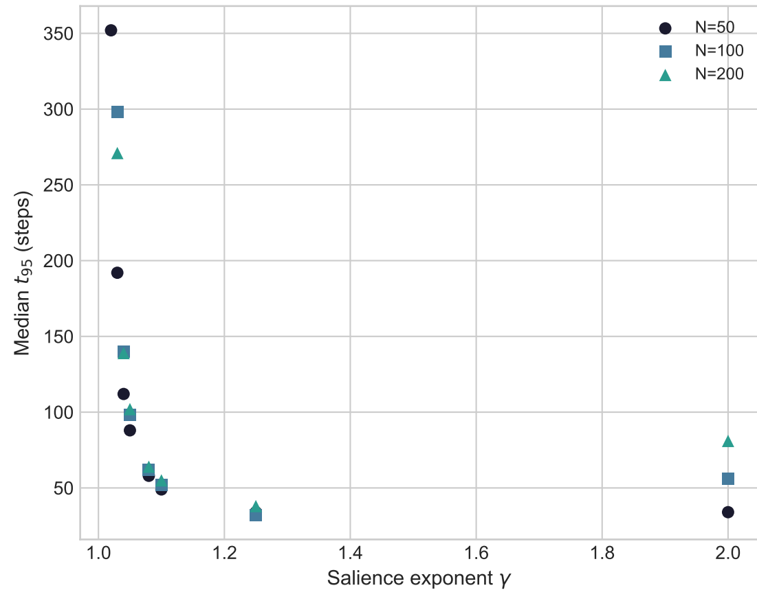
(b) Convergence speed
