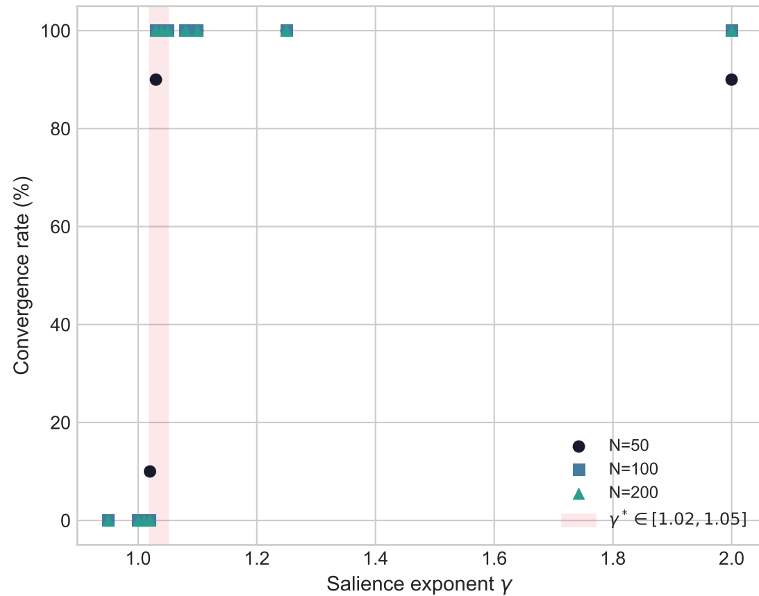
(a) Phase boundary is N-invariant
