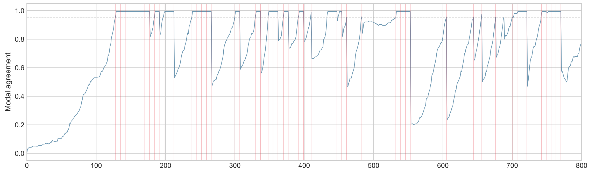
(a) Boundary grinding: N=200 , \gamma=1.05 (54 expulsions in 800 steps)
