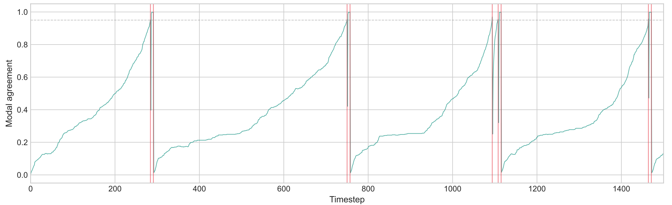
(b) Supercritical bursts: N=500 , \gamma=2.0 (9 expulsions in 1500 steps)
