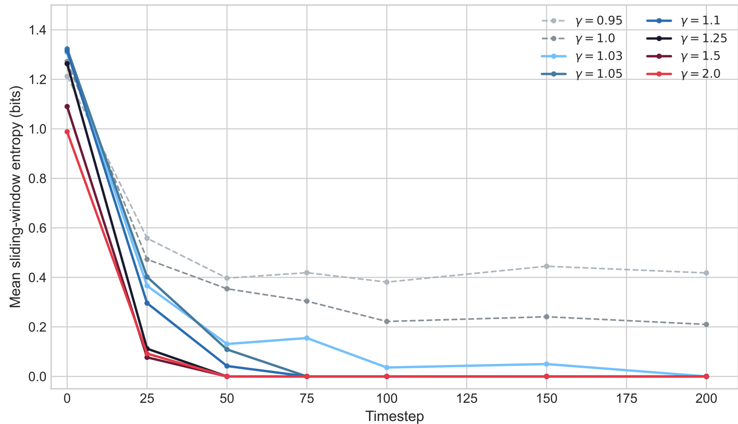
Modal-Target Entropy Decay by Superlinearity
