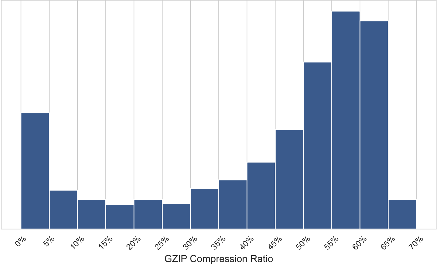
10-Color DNCA GZIP Compression Ratio Distribution
