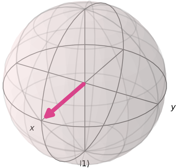
qubit 0 |0\rangle
