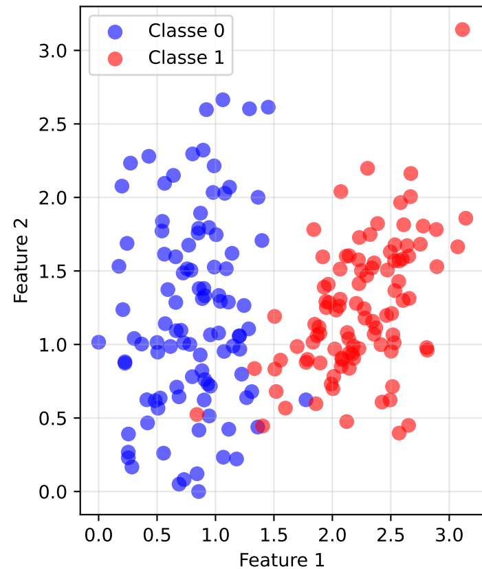
Espaço Original (2D)
