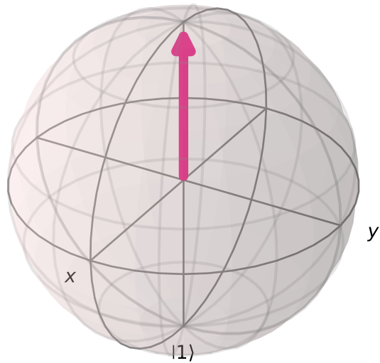
qubit 2 |0\rangle
