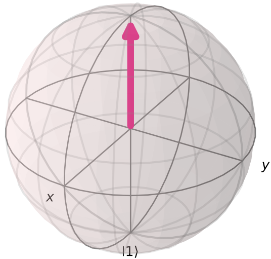
qubit 0 |0\rangle
