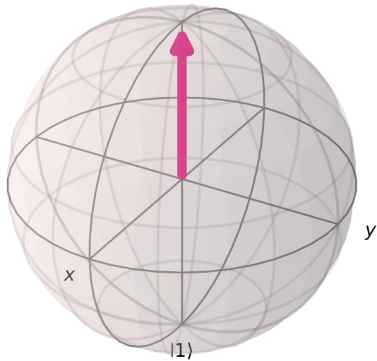
qubit 1 |0\rangle
