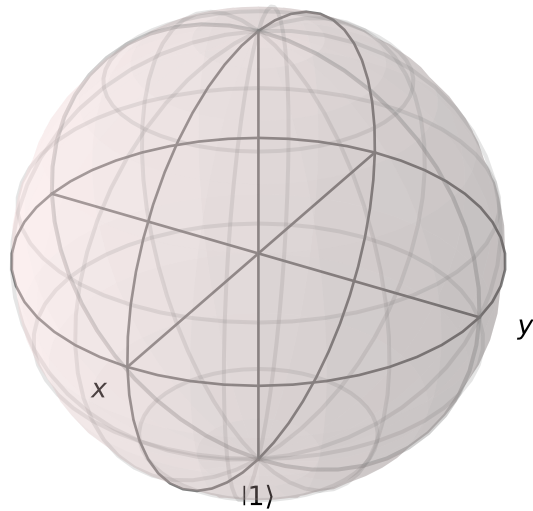
qubit 2 |0\rangle
