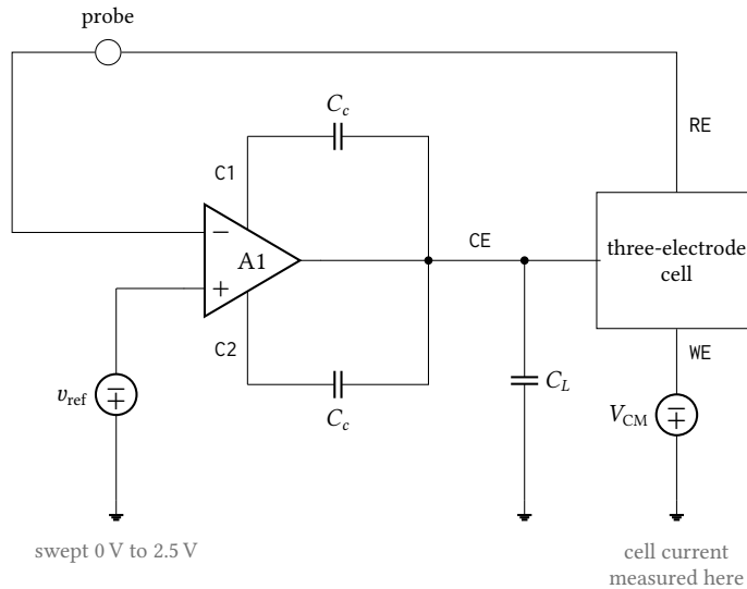
Figure 41: Cell-drive bench. The amplifier drives the counter electrode of a three-electrode cell and closes its loop on the reference electrode, with the commanded potential v_{\text{ref}} swept over the full 0 V to 2.5 V supply range. The working electrode is held at V_{\text{CM}} by an ideal source: no load current is injected, so the cell current is set by the sweep against the cell impedance and is measured in that source, and the regulation errors quoted at \pm 10 \mu\text{A} are read off the sweep at the points where the cell current reaches those values. The probe in the reference-electrode return measures the loop gain with the cell inside the loop; it is not the amplifier's own gain, and the two are tabulated separately. Cell elements are R_{\text{ce}} = R_u = 1 \text{ k}\Omega and R_{\text{ct}} = 10 \text{ k}\Omega in parallel with C_{\text{dl}} = 1 \mu\text{F} (Figure 18), the load is C_L = 5 \text{ pF} , and each external compensation capacitor C_c is 500 fF.
