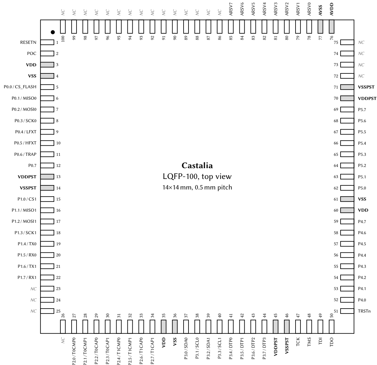
Figure 4: LQFP-100 pinout, top view (14 × 14 mm, 0.5 mm pitch). Each pin is labeled with its pad name and, for GPIO pins, its AF0 (reset-selected) alternate function; power-rail pins are shaded and bold. The full per-pin alternate-function matrix is in Table 5.
