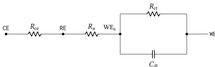
Figure 18: Three-electrode cell model randles_cell, the load the potentiostat actually drives. R_{ce} is the solution resistance from the counter to the reference electrode and R_u the uncompensated resistance from the reference to the working-electrode surface; the interface itself is the charge-transfer resistance R_{ct} in parallel with the double-layer capacitance C_{dl} . Values are given in Table 10. The model is lumped, linear and frequency-independent (no Warburg diffusion term and no potential dependence), so it represents small-signal behaviour about a bias point rather than a full electrochemical response.
