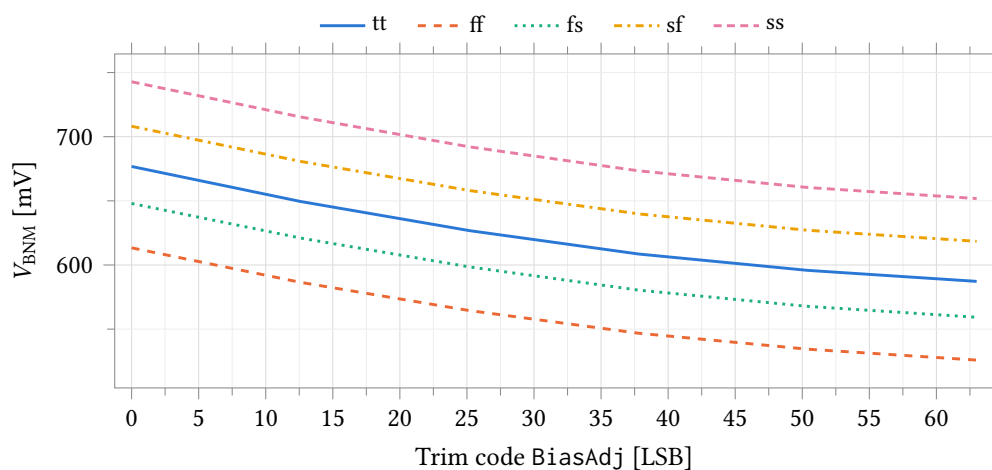
Figure 27: Trim characteristic: V_{\text{BNM}} against the BiasAdj word over all process corners. The bench sweeps the trim word as a continuous variable, so only the six codes 0, 12.6, 25.2, 37.8, 50.4 and 63 are sampled: this is the shape of the trim law, not a per-code characterisation.
