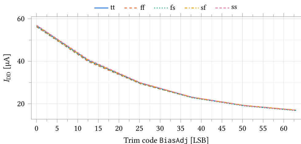
Figure 28: Trim characteristic: quiescent supply current against the BiasAdj word over all process corners, at the same six sampled codes. The current is strongly monotonic in the trim word, falling by a factor of about 3.4 from code 0 to code 63.
