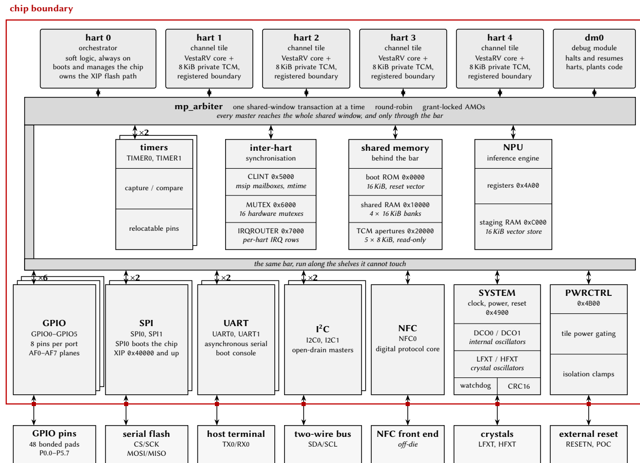
Figure 2: Castalia whole-chip diagram: the bus and the peripherals. One serializing shared-window bus reaches everything on the die, so the mp_arbiter is drawn as the grey bar every block taps — run down the margin and along the lower shelves, because one bar cannot touch three shelves without a tap crossing a box. Masters on top; the pin-facing shelf against the red package boundary, its outside world beyond it; an \times N badge is N instances of one peripheral, not one block. Everything drawn is generated from this configuration.
