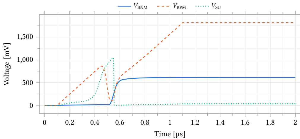
Figure 29: Power-up transient at the typical corner. The start-up node V_{\text{SU}} pulls the core out of its zero-current state, after which both mirror rails settle to their steady-state values.
