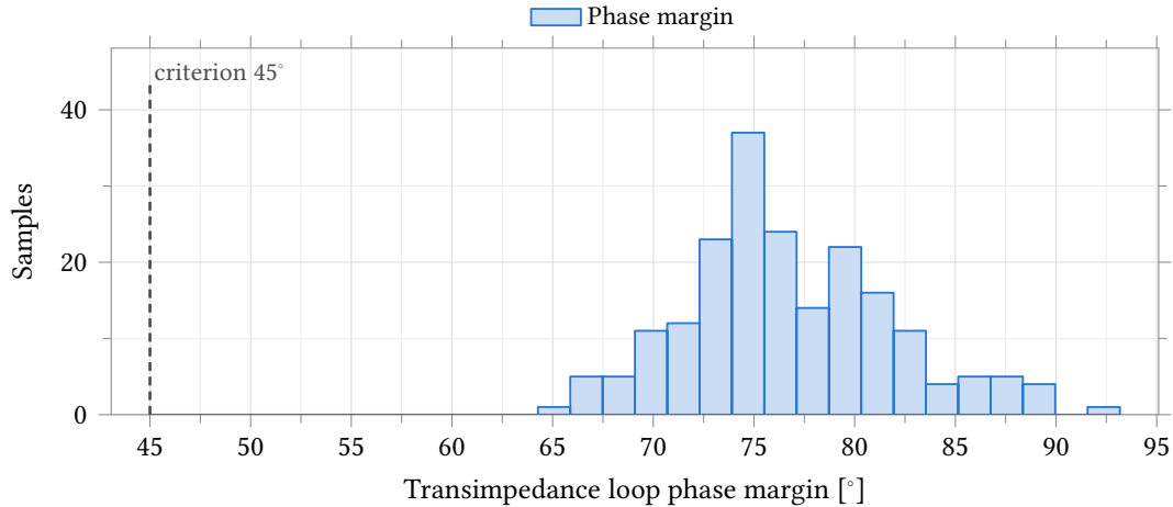
Figure 39: Phase margin of the transimpedance loop, conditions as Figure 38. The loop is measured through the feedback probe of Figure 35 and includes the amplifier, the feedback network and the Randles electrode ( R_s = 100 \Omega , R_{ct} = 1 \text{ M}\Omega , C_{dl} = 100 \text{ nF} ). All 200 samples clear the 45^\circ criterion, minimum 64.7^\circ . The distribution is right-skewed, so percentiles and the extreme sample are quoted in Table 36 rather than \pm 3\sigma .
