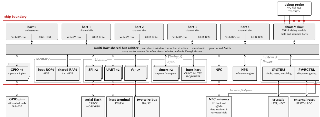
Figure 3: Castalia whole-chip diagram, flat companion to Figure 2: the same generated content on one bus bar and one rank. The bar is the mp_arbiter entity of the RTL. Every master taps it from above and every peripheral taps it from below, straight up, so there is one bus in this drawing and no second segment of it. A hart box is split into the two things the tile is built from – the VestaRV core and its private TCM. Each of those TCMs is also windowed read-only into the shared map (Section 3), which is why the rank carries no aperture box of its own. Peripheral boxes carry a name and one line only; the addresses are in Section 3, and a \times N in a title – with the offset squares stacked behind the box – is N instances of one peripheral, not one block. The rank is grouped by type: the grey headings, and the thin outlines round every type that has more than one box or compartment, are organisation only – every block under them is an arbiter slave in its own right, tapping the bar on its own wire. Every off-chip partner hangs on a straight vertical wire dropped from the tap above it, entering the partner’s top edge off-centre where the partner had to be nudged aside. The JTAG/debug column and the NFC block are drawn solid in every build, whether or not this configuration contains them: what a given build actually has is the debug.enable and peripherals.nfc knobs of Table 1, and the JTAG column prints debug builds only in the box where this build has no debug module in it. The one stroke in the drawing that still changes with the configuration is the harvested-supply rail, drawn dashed where this build does not run the chip off the field. The Debug Module is one more master on the bar, reached over five JTAG pins from an off-chip probe, and is present in debug-enabled builds only. NFC has two roles and this view draws both: its digital core reads the tag through the bar like any peripheral – the RF front end is off-die – and on a field-powered board the harvested field is the chip’s supply , which is the heavy grey rail running along the off-chip band into PWRCTRL’s PGOOD and boot-strap taps, whose boot gate holds every hart in reset until that supply is good. Everything drawn is generated from this configuration.
