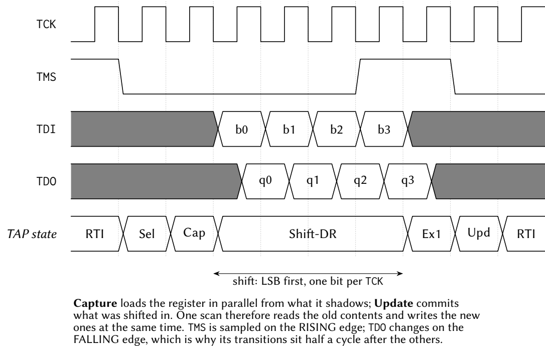
Figure 11: One four-bit data-register scan. The state row is the sequence the port walks under the TMS pattern above it. Data is shifted least-significant bit first, one bit per TCK; TDI is sampled on the rising edge and TDO changes on the falling one, which is why the two rows are offset by half a cycle. A real scan is 32 or 41 bits wide rather than four, but the shape is exactly this.
