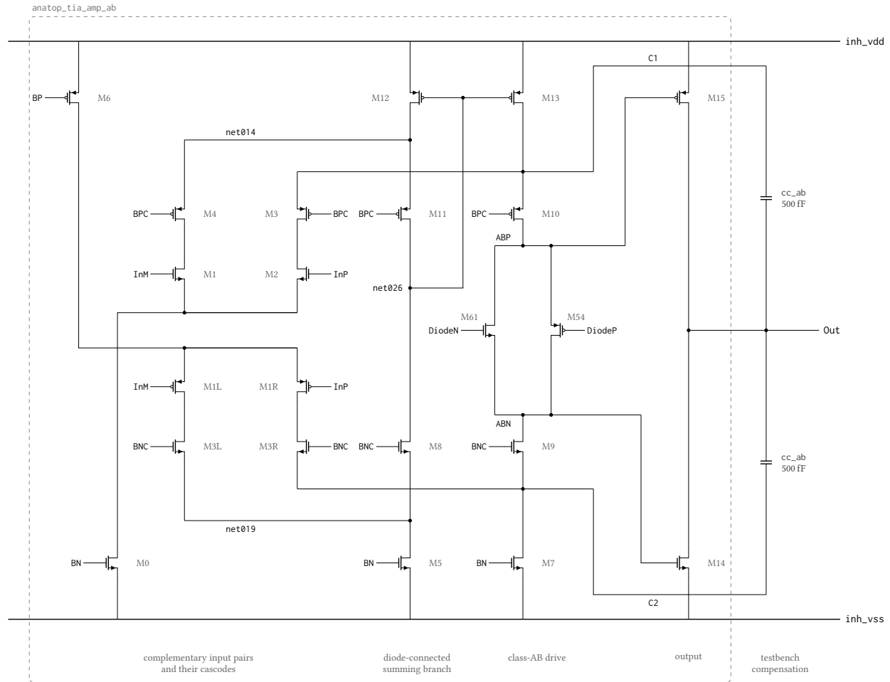
Figure 51: Signal-path topology of the class-AB amplifier anatop_tia_amp_ab , drawn from its netlist. The complementary pairs M1/M2 (NMOS, tail M0 ) and M1L/M1R (PMOS, tail M6 ) fold into two cascode branches; the InM side terminates in the diode-connected branch M12-M11-M8-M5 , whose summing node net026 sets M13 , which restates that current into the InP branch, and the floating pair M54/M61 holds ABP above ABN so both output devices M15 and M14 are actively driven. C1 and C2 are the common source nodes of the PMOS cascodes M10/M3 and of the NMOS cascodes M9/M3R , brought out as pins; the two cc_ab capacitors that return them to Out sit outside the cell boundary (dashed) in the testbench, 500 fF per side. Simplified: the enable switch and its four power-down devices, and the bias generator that develops DiodeN/DiodeP , are omitted, so 22 of the cell's 34 transistors are drawn; BP/BPC/BN/BNC are the enable-gated forms of the bp!/bpc!/bn!/bnc! globals and device dimensions are not shown. Identically labelled nets are connected; wires crossing without a filled dot are not.
