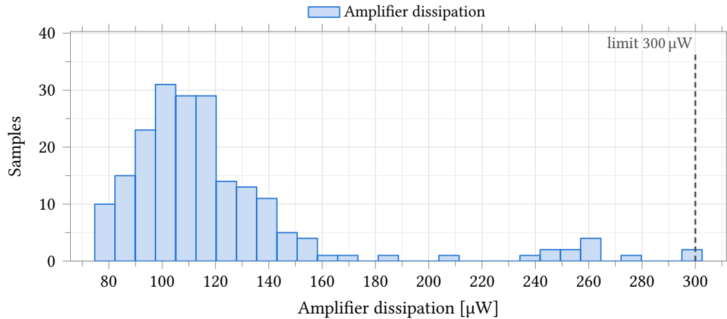
Figure 57: Amplifier dissipation at the DC operating point. Process and mismatch (castalia_pm_25), 25 °C, 200 samples, seed 12345, LDS sampling, BiasAdj = 37, 2.5 V, both inputs at v_{cm} , no load current; at this open-loop operating point the output rests near v_{ss} . The distribution is bimodal: 187 of 200 samples lie between 75 \mu W and 170 \mu W (median 111.8 \mu W) and 13 converge to a second DC solution branch of the degenerate open-loop operating point, up to the worst sample at 302.5 \mu W against the 300 \mu W limit entered on the test. Mean \pm 3\sigma is not meaningful for this shape and is not quoted. The figure is the amplifier instance alone and excludes the shared bias generator.
