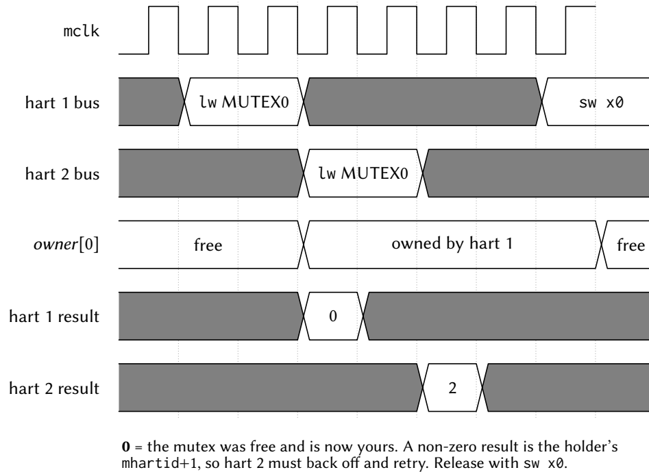
Figure 71: Two harts racing for the same mutex. The arbiter serializes the two claim reads, so the return-old-and-claim happens atomically with no retry loop: the hart the arbiter serves first reads 0 and thereby owns the mutex, and the other reads the winner's marker (mhartid + 1) and must back off.
