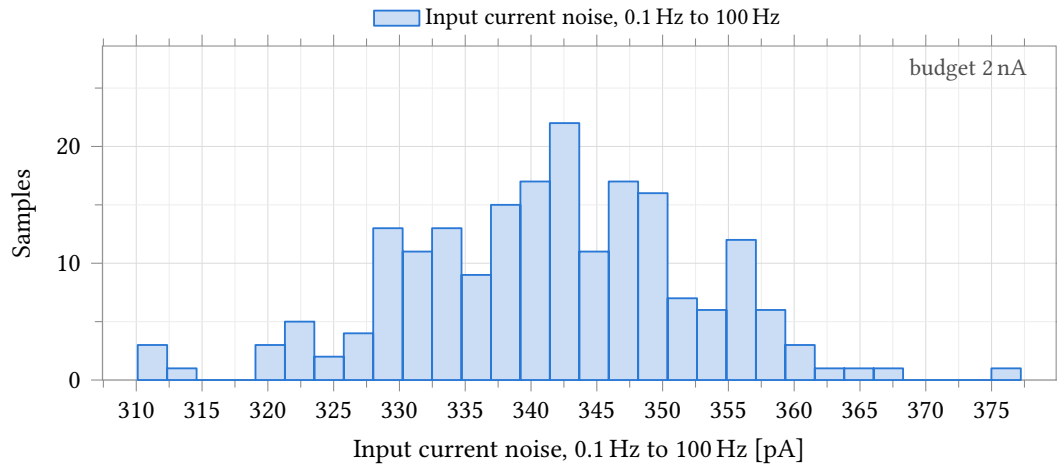
Figure 56: Input-referred current noise integrated 0.1 Hz to 100 Hz, conditions as Figure 54. Output noise divided by R_f , from a noise analysis that runs 0.1 Hz to 10 kHz at 20 points per decade. The 2 nA budget entered on the test is about six times the measured value and is annotated at the axis edge rather than drawn, so that the 310 pA to 377 pA spread stays legible. The figure scales inversely with the selected gain tap.
