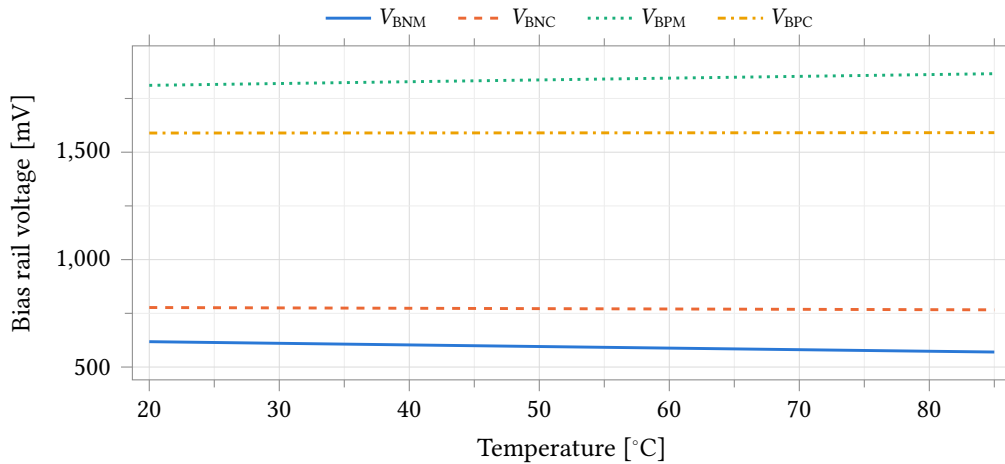
Figure 16: The four local bias rails against temperature at the typical corner. V_{BNM} and V_{BNC} are referred to vss! ; V_{BPM} and V_{BPC} sit near the supply.
