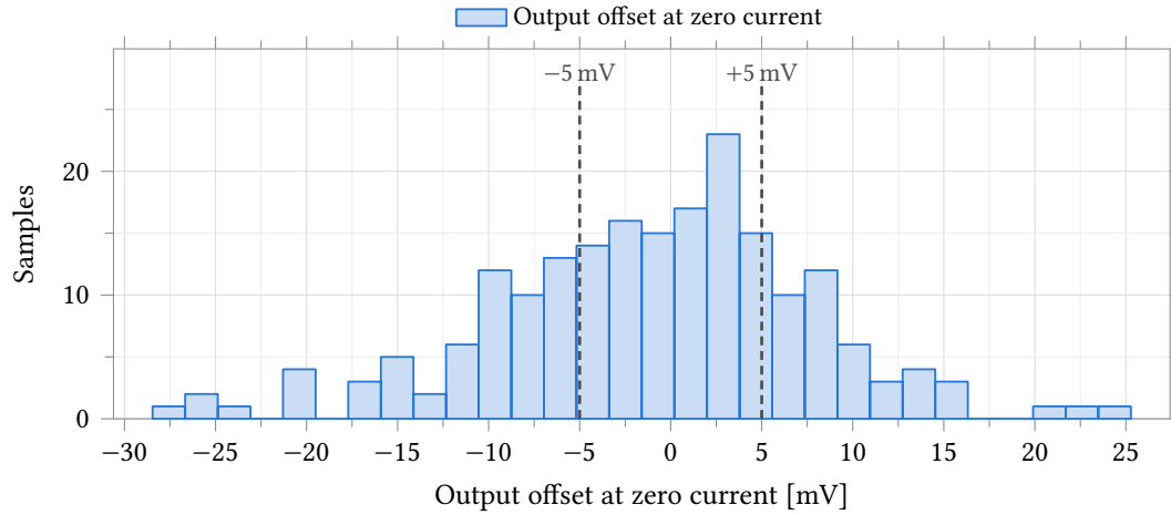
Figure 54: Output offset at zero electrode current, referred to v_{cm} . Process and mismatch (castalia_pm_25), 37 °C, 200 samples, seed 12345, LDS sampling, R_f = 560\text{ k}\Omega , C_f = 22\text{ pF} , C_L = 5\text{ pF} , C_c = 500\text{ fF} , BiasAdj = 37, 2.5 V. The rules are the \pm 5\text{ mV} limits entered on the test. \sigma = 8.91\text{ mV} (sample deviation, as in every table of this section); 96 of 200 samples lie within the limits, 5.3 % across four independent channels. Statistics are in Table 48.
