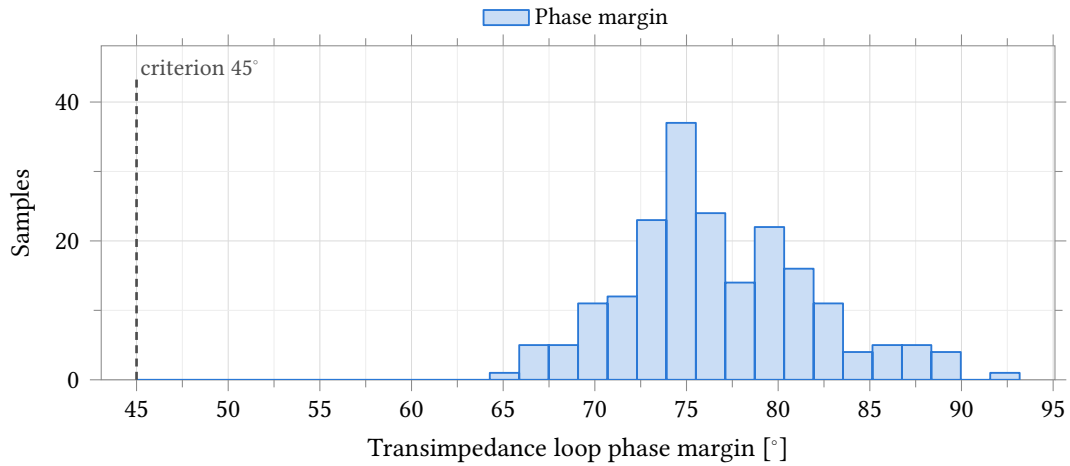
Figure 55: Phase margin of the transimpedance loop, conditions as Figure 54. The loop is measured by stb through the IPRB_F probe and includes the amplifier, the feedback network and the randles_cell electrode ( R_s = 100\ \Omega , R_{ct} = 1\ \text{M}\Omega , C_{dl} = 100\ \text{nF} ). All 200 samples clear the 45^\circ criterion, minimum 64.7^\circ . The distribution is right-skewed, so percentiles and the extreme sample are quoted in Table 50 rather than \pm 3\sigma .
