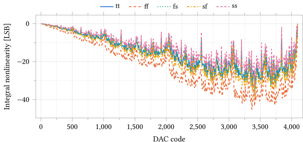
Figure 70: Integral nonlinearity against code over five process corners with the ladder referenced to V_{ddDac} from the supply block, zero external load, 25 °C. Endpoint-line INL as in Figure 66; the vertical scale is tens of LSB, not tenths. The bow reaches −37.1 LSB at tt (code 3413) and −45.1 LSB at ff (code 3365) and tracks the reference droop of Figure 69 scaled by code. Dividing each code’s output by the reference measured at that code removes it and leaves 0.43 to 0.45 LSB (Table 73), so the ladder is unchanged from the ideal-rail case.
