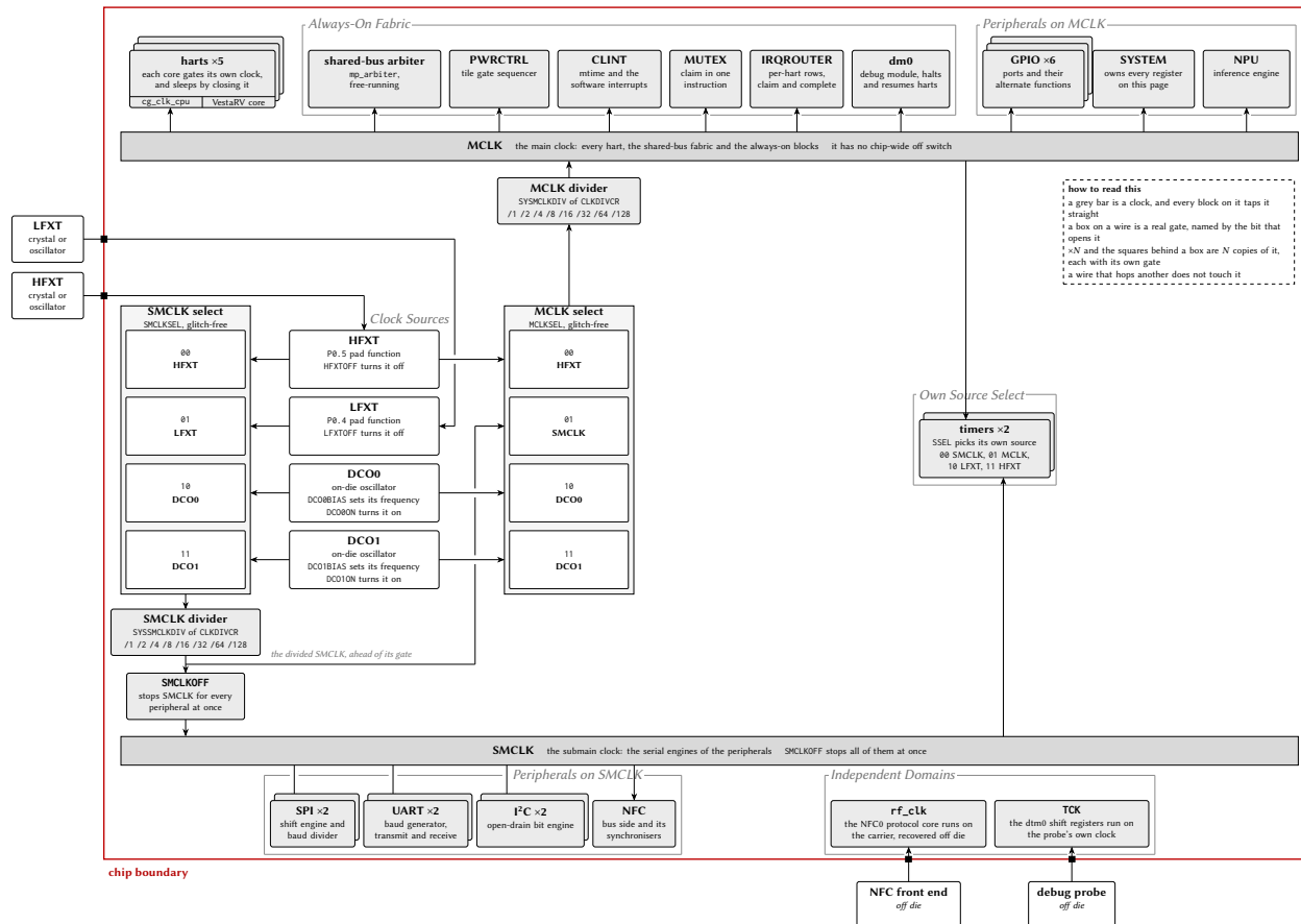
Figure 91: The MCU clock system, generated from this configuration. The layout is a mirror: the sources stand in one column, in the order SMCLKSEL enumerates them, the SMCLK chain runs left out of that column and down into its own bar, and the MCLK chain runs right out of it and up into its own, so every source leg is a straight horizontal at its own row. Each select box prints every code it has, with the name of what that code picks, and those rows are built from the register model itself rather than drawn by hand. One code is not a source: MCLKSEL 01 takes SMCLK, tapped after the SMCLK divider and before the SMCLKOFF gate, which is why stopping SMCLK never stops MCLK; it is the one wire in the drawing that has to leave its row, and it hops the legs it crosses rather than touching them. A source that either select is using stays enabled whatever its own bit says. Every block on a bar taps it straight up or straight down; the sleep gate is drawn where the hardware puts it, inside each core, so the stack of five harts is a stack of five gates. A block with a select of its own names every code it has and taps the two bars it can reach, so the crystal sources it may also pick are named in its box rather than drawn as two more wires across the page. The blocks under Independent Domains are on neither bar: they are clocked from outside this tree entirely, and SYSCLKCR does not reach them. The register interface of every peripheral is clocked from MCLK even where its engine runs on SMCLK, which is why a peripheral stays readable with SMCLK stopped.
