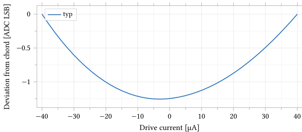
Figure 63: Drive nonlinearity of the bottom code ( N = 0 , R \approx 19.6 k \Omega ): voltage deviation from the endpoint chord over \pm 90 % of full scale ( \pm 40 \mu A), typical corner, expressed in 1.592 mV ADC LSB. All ten bypass gates are closed at this code and carry the full signal current; their on-resistance rises with the terminal's excursion from V_{CM} , so the chord — pinned at the sweep endpoints where that excursion is largest — overestimates the mid-range voltage by up to 1.25 LSB, and the deviation is bowl-shaped with a slight skew from the gates' voltage asymmetry. The same measurement at N = 63 and N = 319 , where the ladder dominates and current is 20–100 \times smaller, stays below 0.004 LSB and is tabulated, not plotted.
