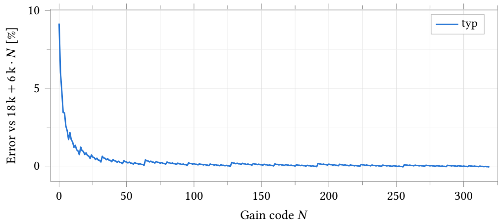
Figure 62: Typical-corner deviation from the ideal code law. The +9.2 % at N = 0 is the series resistance of the ten closed bypass switches (1.65 k \Omega , about 165 \Omega each), which decays as 1/R once real ladder segments dominate; by N = 319 the error is -0.063 %. The ripple is the carry structure: at each binary carry and at each thermometer seam the set of closed switches changes, so the R_{on} term steps while the ladder term is exact.
