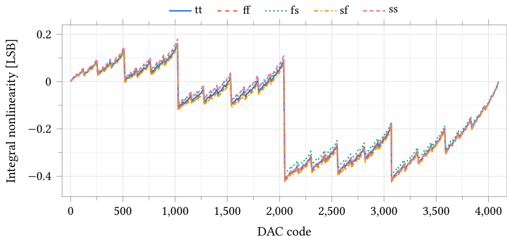
Figure 66: Integral nonlinearity against code over five process corners, ladder on an ideal 2.5 V rail, 25^\circ\text{C} , \text{reltol} = 1 \times 10^{-6} . INL is taken from the endpoint line through each corner's own zero- and full-scale outputs, so it is zero at codes 0 and 4095 by construction. The positive extreme is code 1023, +0.15 to +0.18 LSB; the negative extreme is shared by the major carries at codes 2048 and 3072, which sit within 0.006 LSB of each other at -0.39 to -0.43 LSB at every corner. The code of each extreme is the same at all five corners: the shape is set by the ladder, not by the process. Corner run, no device mismatch — R - 2R linearity is a matching property, so this envelope is the systematic term alone.
