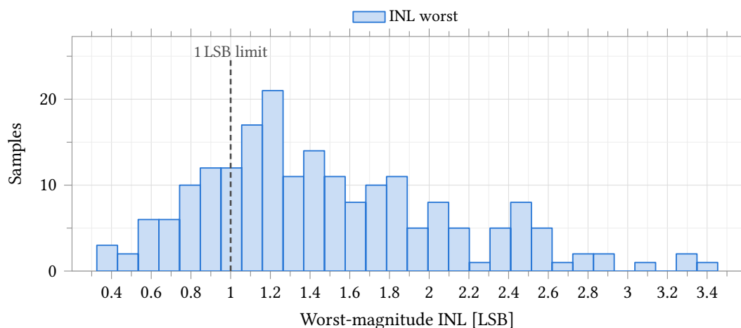
Figure 72: Integral nonlinearity of the R -2 R ladder driven from an ideal 2.5 V reference. Process and mismatch , model section castalia_pm_25 , 200 samples, seed 12345, low-discrepancy sampling, 25 °C, all 4096 codes. The dashed rule is the 1 LSB limit entered on the test; 42 of 200 samples fall inside it and the worst reaches 3.453 LSB. The distribution is right-skewed (Fisher skew +0.74), so Table 74 quotes the median and percentiles rather than \text{mean} \pm 3\sigma . LSB size, full scale and gain error are fixed to a part in 10^6 on this bench (Table 75), so the whole of this spread is resistor mismatch in the ladder and none of it is the reference.
