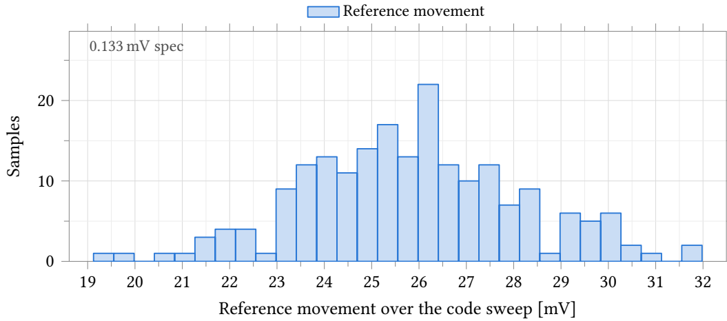
Figure 74: Peak-to-peak movement of the DAC reference V_{ddDac} across the 4096-code sweep, with the ladder referenced to the on-chip supply block instead of an ideal rail. Process and mismatch , castalia_pm_25 , 200 samples, 25 °C, no external load on V_{ddDac} . The quarter-LSB budget of 133 \mu V entered on the test sits about 200 times below the data, so it is annotated at the left axis edge rather than drawn and the distribution is not compressed into a single bar; the closest sample misses it by a factor of 144. Meeting it needs the supply’s output impedance down by a factor of 193, to about 5 \Omega , against 894 \Omega small-signal (Table 83) and 1133 \Omega as a 0 \mu A to 100 \mu A chord (Table 79).
