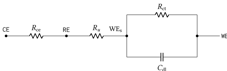
Figure 19: Three-electrode cell model randles_cell , the load the potentiostat actually drives. R_{ce} is the solution resistance from the counter to the reference electrode and R_u the uncompensated resistance from the reference to the working-electrode surface; the interface itself is the charge-transfer resistance R_{ct} in parallel with the double-layer capacitance C_{dl} . Values are given in Table 12. The model is lumped, linear and frequency-independent (no Warburg diffusion term and no potential dependence), so it represents small-signal behaviour about a bias point rather than a full electrochemical response.
