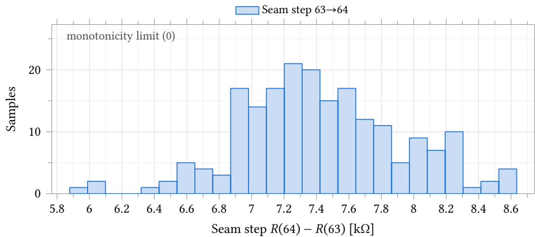
Figure 64: Per-sample step across the first thermometer seam (code 63 to 64: one 64-unit segment switches in while all six binary segments switch out), the code transition most exposed to mismatch. Mismatch only , model section castalia_pm_25 , nominal process, 200 samples, seed 12345, low-discrepancy sampling, 25 °C. Mean 7.42 k \Omega , \sigma = 504 \Omega , worst sample 5.88 k \Omega – 14.7\sigma above the monotonicity limit at zero, so no realistic mismatch closes the seam.
