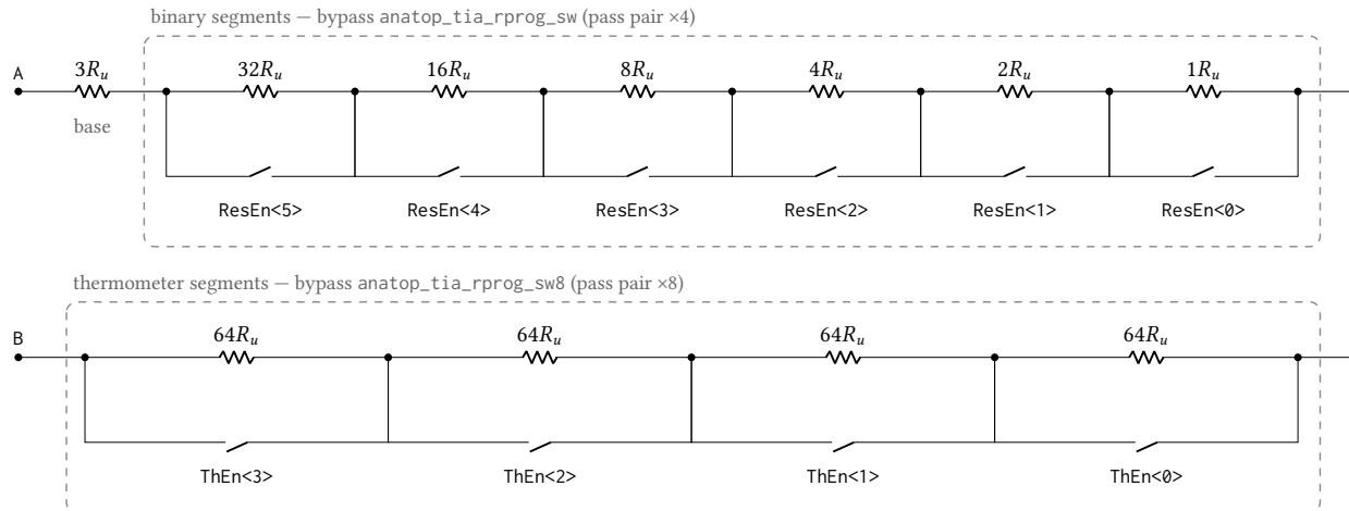
Figure 60: Segment and bypass-switch structure of anatop_tia_rprog, transcribed from the executed spec-run netlist. The unit R_u is one series poly resistor; from terminal A the chain runs through the never-switched three-unit base, the six binary-weighted segments of 32 down to 1 unit, and the four identical 64-unit thermometer segments to terminal B. Each switched segment is shunted by a CMOS transmission gate with a local inverter: the control pin EnBar is the ResEn/ThEn bit itself and drives the PMOS pass gate directly and the NMOS pass gate through the inverter, so a bit at 1 turns both pass devices off and inserts the segment. The pass pair has multiplicity 4 in the binary switch ( _sw ) and 8 in the thermometer switch ( _sw8 ), which halves the thermometer gates' on-resistance where up to six binary gates close at a seam. Three grounded dummy units accompany the 322 active units for matching.
