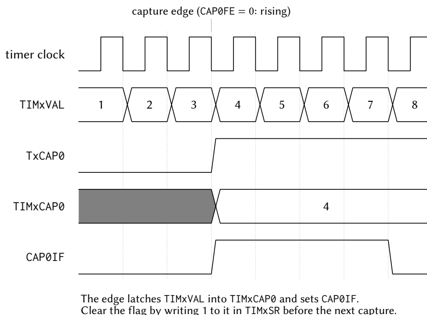
Figure 90: Input capture. The selected edge on TxCAP0 latches the live TIMxVAL into TIMxCAP0 and sets CAP0IF; the flag must be cleared by writing 1 to it in TIMxSR before the next capture event.
