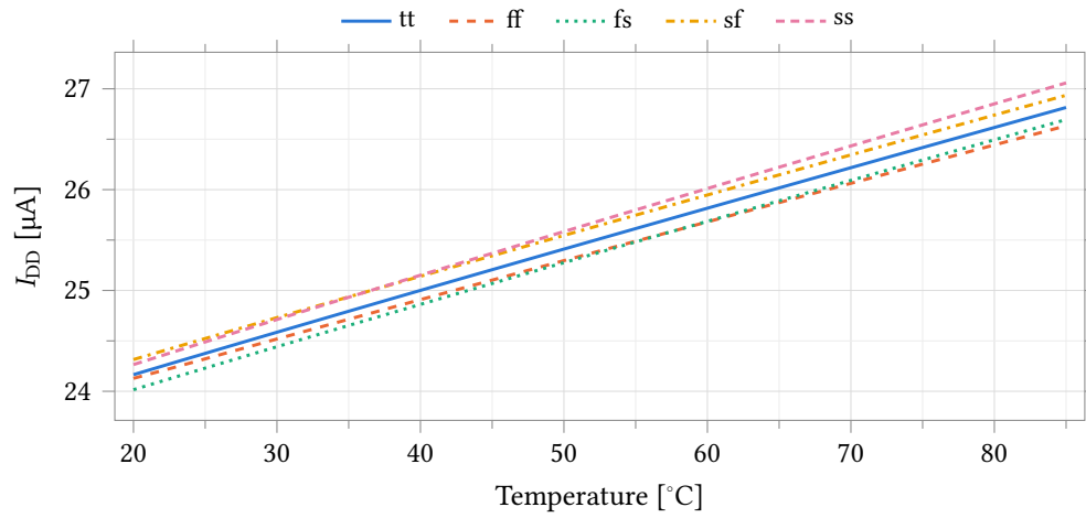
Figure 8: Quiescent supply current of the bias generator against temperature over all process corners.
