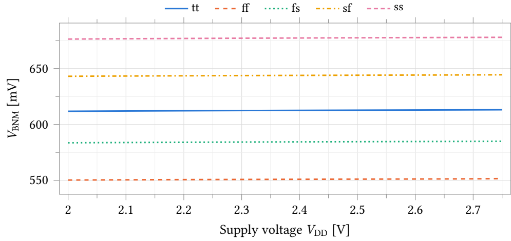
Figure 9: Supply rejection of the NMOS mirror bias: V_{\text{BNM}} against V_{\text{DD}} over all process corners.
