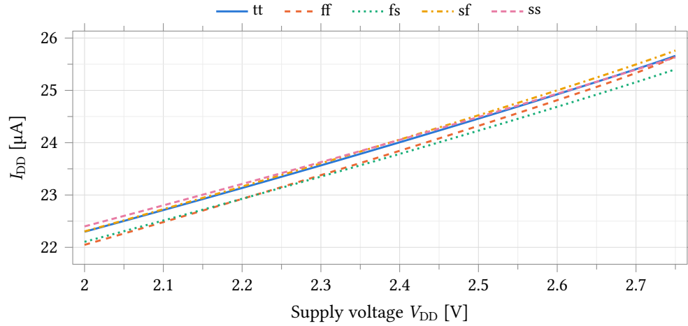
Figure 10: Quiescent supply current against supply voltage over all process corners.
