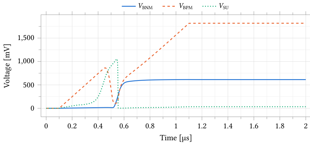
Figure 13: Power-up transient at the typical corner. The start-up node V_{SU} pulls the core out of its zero-current state, after which both mirror rails settle to their steady-state values.
