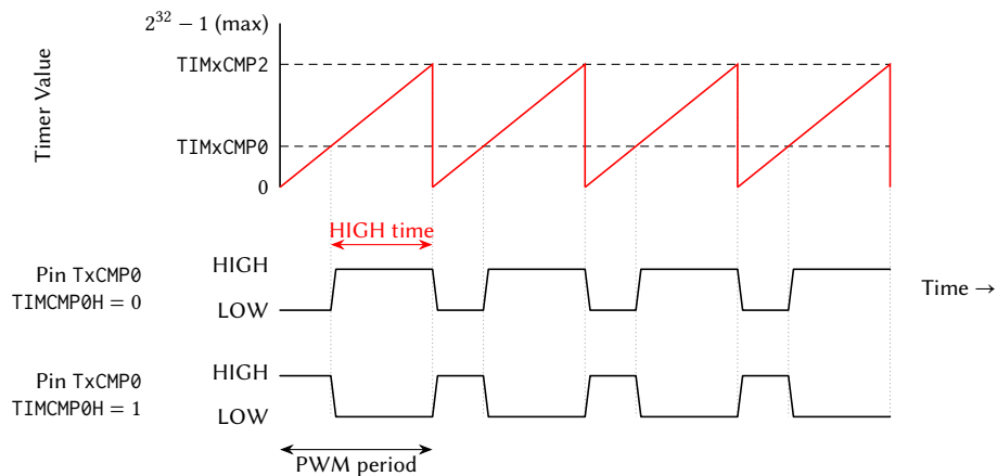
Figure 23: Timer Output Compare and PWM Operation
