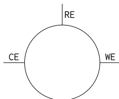
Figure 19: Three-electrode cell model, the load the potentiostat actually drives, shown as the symbol used throughout this chapter. It is a lumped linear network between the counter, reference and working electrodes; its elements and their values are given in Table 12. The model is frequency-independent (no Warburg diffusion term and no potential dependence), so it represents small-signal behaviour about a bias point rather than a full electrochemical response.
