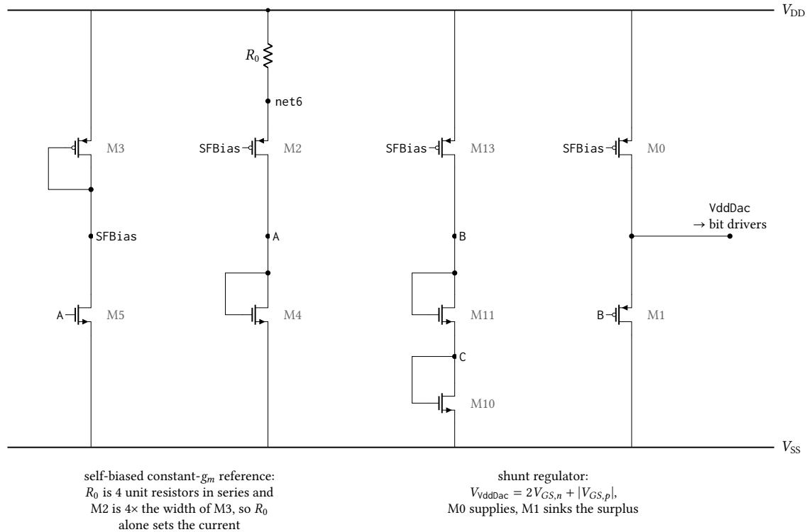
Figure 72: Core of anotop_pixel_dac_psu , the shunt regulator that generates the VddDac rail the ladder uses as its reference, transcribed from the LoadRegTB netlist. The self-biased constant- g_m reference on the left sets SFBias ; M_{13} drives that current through the stacked diodes M_{11} and M_{10} to hold B two gate-source voltages above V_{SS} , and M_1 sinks whatever of M_0 's current the ladder leaves, clamping VddDac one PMOS gate-source voltage above B : 2.177 V unloaded from a 2.5 V rail. There is no error amplifier, so load regulation is set by M_1 's g_m alone. The five start-up and enable devices — the weak pull-up and its two kick devices on SU , the shutdown pull-up on SFBias and the En inverter — are omitted; none carries current once the loop is running. Device dimensions are proprietary and are not stated.
