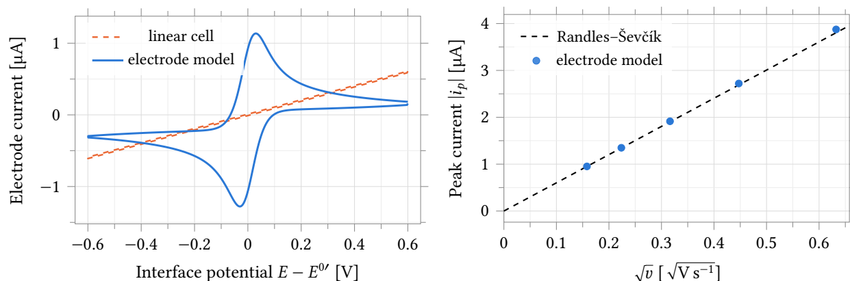
Figure 21: Standalone validation of the electrode model against closed-form voltammetry, ideal potential source, model defaults of Table 13 with R_s = 500 \Omega and C_{dl} = 0.2 \mu F in series and in parallel respectively, 25^\circ C . Left: current against interface potential over a \pm 0.6 V triangular sweep at 50 mV s^{-1} , second cycle, for the nonlinear model (solid) and for the linear cell of Section 8.1 driven identically (dashed, R_{ct} = 1 M\Omega ); the linear response is a ramp with its extrema pinned at the switching potentials — its C_{dl} box is only 20 nA wide at this scan rate and invisible here — while the nonlinear one peaks 30 mV either side of E^{0'} and decays afterwards. Right: peak cathodic current of the first scan against \sqrt{v} over 25 mV s^{-1} to 400 mV s^{-1} , against the Randles-Ševčík line, of slope 6.015 \mu A per \sqrt{V s^{-1}} ; the two panels use different cycles because Randles-Ševčík describes the first scan into an undepleted bulk, while the second cycle is the repeatable steady response and sits 3 % to 5 % below it. Numbers in Table 14.
