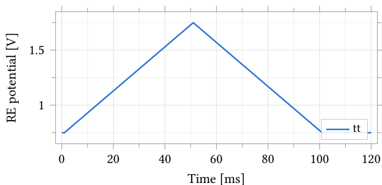
Figure 54: Commanded reference-electrode potential against time for the triangular voltammetry sweep, typical process point, 37^{\circ}\text{C} , R_f = 35\text{ k}\Omega , R_{ct} = 1\text{ M}\Omega electrode. Paired with the current response of Figure 53.
