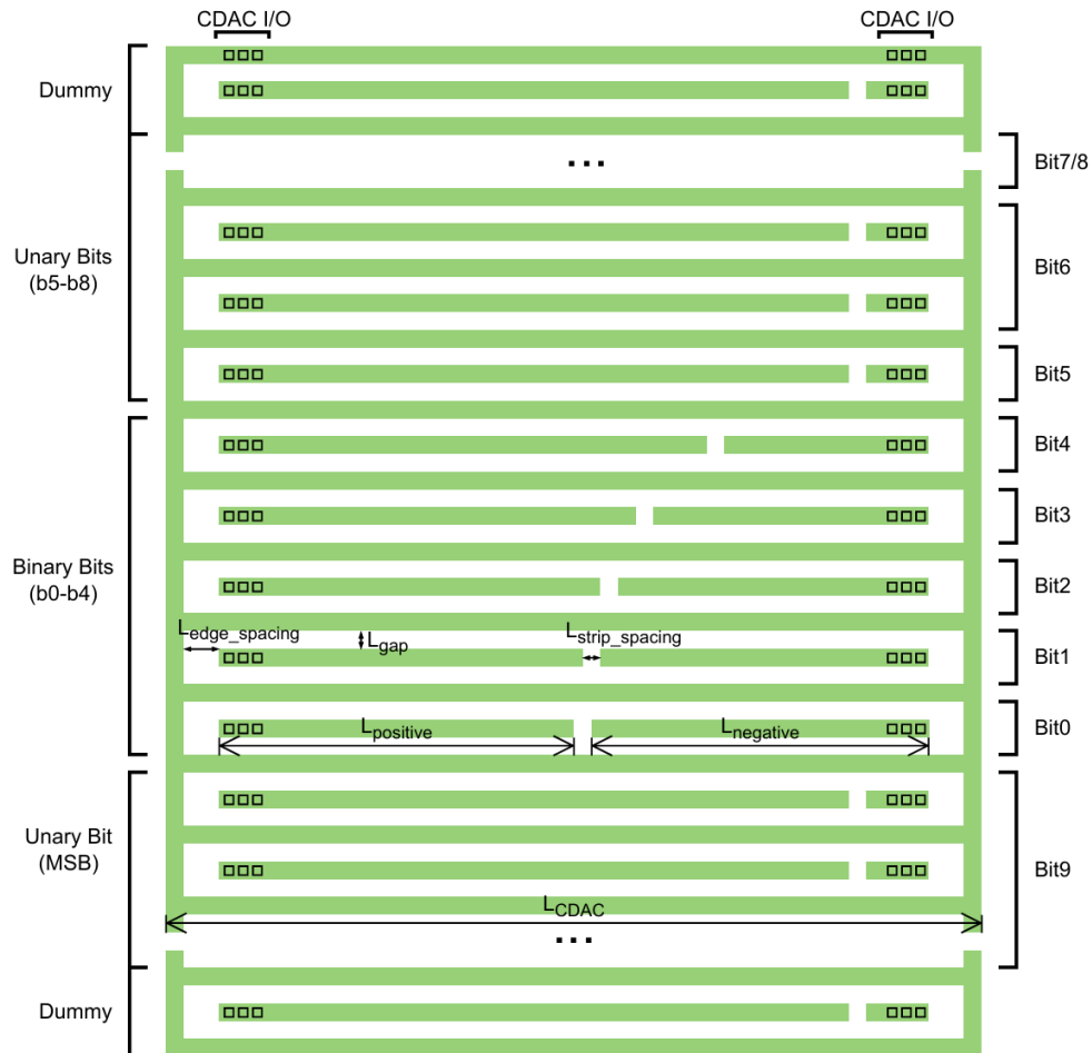
Figure 59: Floor plan of the 10-bit segmented capacitor array of anatop_pixel_adc . The five lower bits b0–b4 are binary-weighted within single strips, each strip split into a positive and a negative section whose boundary sets the weight; the upper bits b5–b8 and the MSB b9 are unary, built from repeated identical strips, and every row terminates in CDAC I/O at both ends. Unary segmentation of the large weights makes their ratio a count of identical unit strips rather than the dimension of one large device, so it is set by matching; the dummy rows at the top and bottom of the array give the outermost active strips the same local surroundings as interior ones. The array exists only in layout, which is why this section’s data is taken from an extracted netlist.
