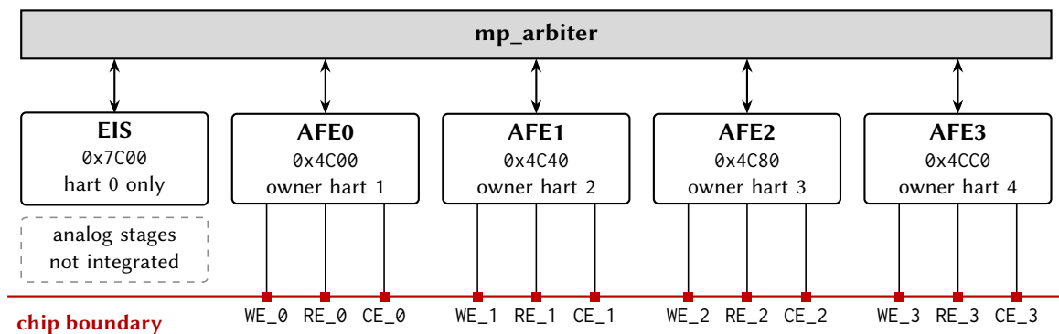
Figure 23.3: Analog front-end connectivity: each AFE site answers its owning hart and hart 0, the EIS site answers hart 0 only, and three electrode pads per site leave the die.
