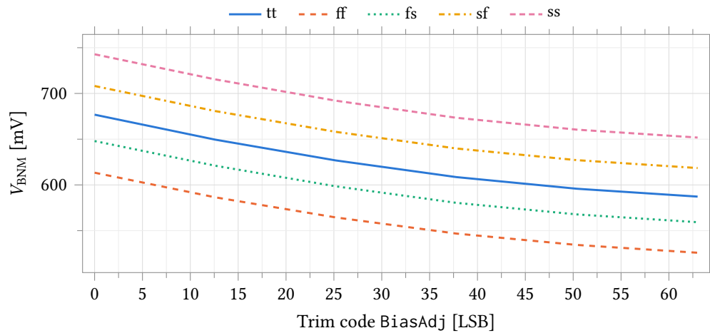
Figure 14: Trim characteristic: V_{\text{BNM}} against the BiasAdj word over all process corners. The bench sweeps the trim word as a continuous variable, so only the six codes 0, 12.6, 25.2, 37.8, 50.4 and 63 are sampled — this is the shape of the trim law, not a per-code characterisation.
