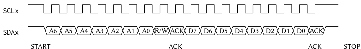
Figure 47: One I2C byte write on the wire: START, the 7-bit address and direction bit, the addressed device's ACK, one data byte, its ACK, then STOP. START and STOP are the two transitions of SDAx that occur while SCLx is high; every data bit is stable across the SCLx high period.
