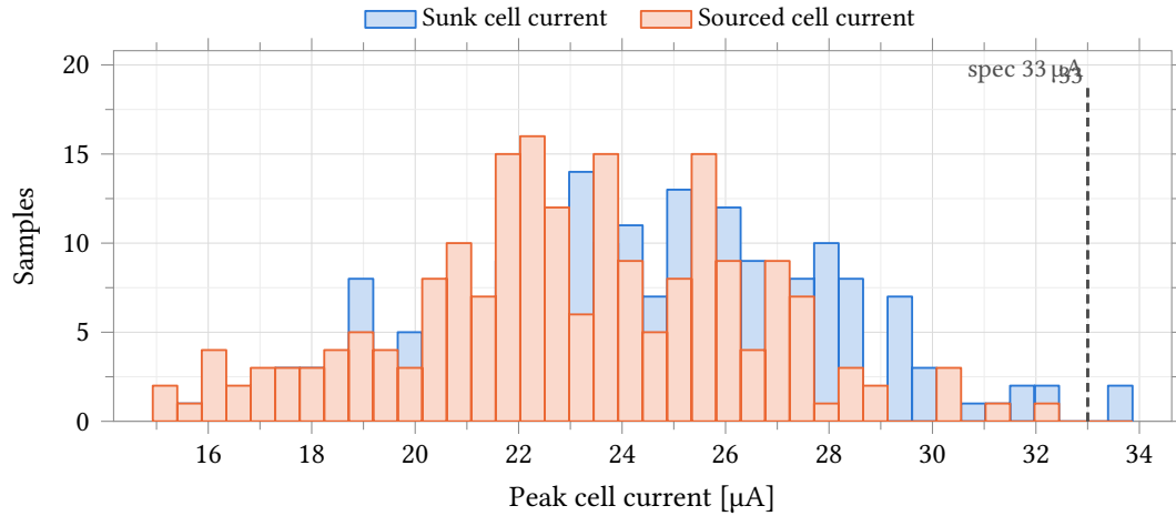
Figure 22: Peak current delivered into the cell, sinking and sourcing, over 200 process-and-mismatch samples. The two distributions overlap almost completely: mean source/sink imbalance is 6.4 %. Absolute drive falls short – 23.0 \mu\text{A} sourcing and 24.4 \mu\text{A} sinking against a 33 \mu\text{A} target, reached by 2 of 400 measurements. Roughly 1 V of headroom is left unused at each rail (Table 17), so the limit is current, not swing.
