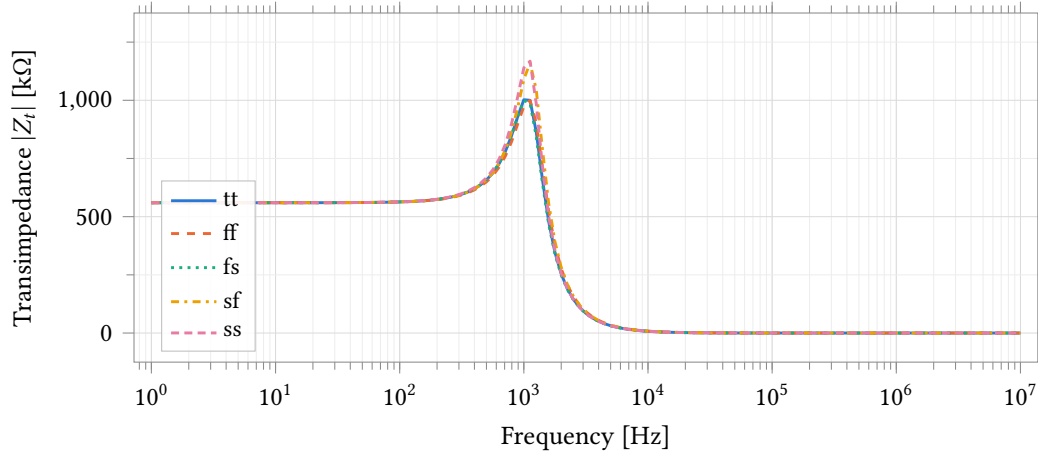
Figure 33: Transimpedance |Z_t| against frequency over the five corners, at maximum gain ( R_f = 560 \text{ k}\Omega ) with 1 \mu\text{F} of double-layer capacitance at the working electrode. Flat at 560 \text{ k}\Omega to about 200 \text{ Hz} , it peaks to 1.00 \text{ M}\Omega to 1.17 \text{ M}\Omega near 1 \text{ kHz} . The peak is a marginally stable loop caused by C_{dl} rolling the feedback factor off from 0.28 \text{ Hz} , not by the amplifier.
