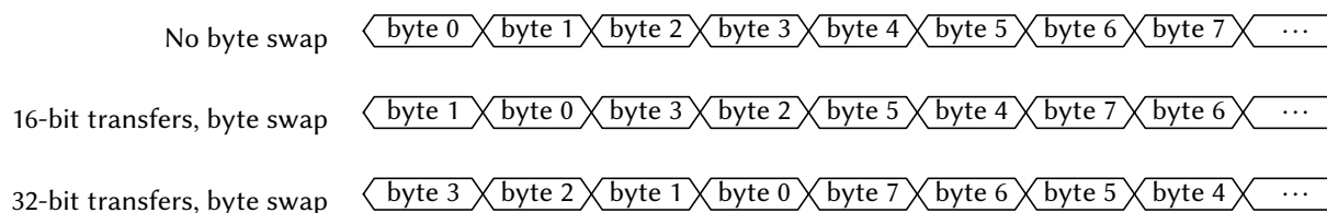
Figure 38: SPI Byte Ordering
