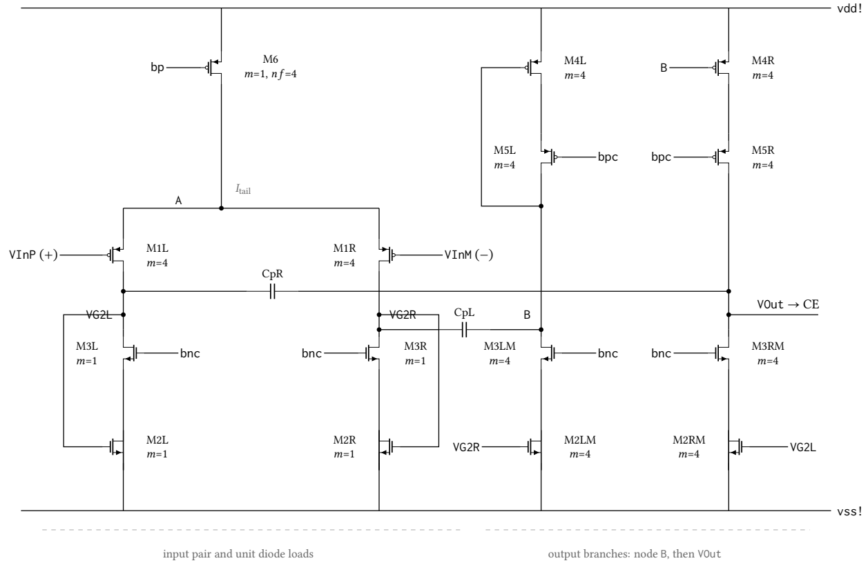
Figure 18: Control amplifier core: a symmetric current-mirror (mirrored) OTA with a PMOS input pair, drawn in the same arrangement as the Virtuoso cellview — input pair and its two unit diode loads on the left, the two output branches on the right. Each input device steers part of I_{tail} into a unit diode ( m=1 ); a mirror four times larger then restates it, the extttVG2L half directly onto extttVOut and the extttVG2R half into node extttB, where the PMOS mirror inverts it and returns it to extttVOut so the two halves add. Both output devices are cascoded. extttCpL and extttCpR damp the mirror poles. Identically labelled nets are connected; matching dummies are omitted.
