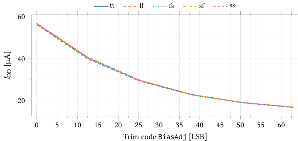
Figure 15: Trim characteristic: quiescent supply current against the BiasAdj word over all process corners, at the same six sampled codes. The current is strongly monotonic in the trim word, falling by a factor of about 3.4 from code 0 to code 63.
