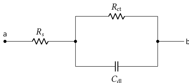
(b) randles_electrode
