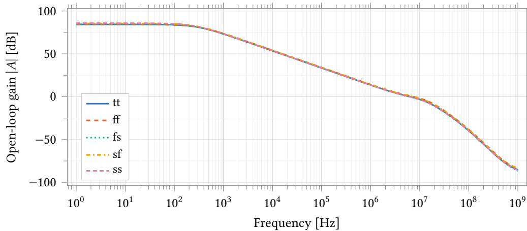
Figure 28: Open-loop gain over the five process corners, by stb through the feedback probe with the amplifier in unity feedback and a 5 pF load. Miller compensation gives a single-pole roll-off from 290 Hz to a 6.2 MHz to 7.6 MHz crossover. This is the amplifier alone; the loop that closes around the electrode is not this well behaved (Figure 33).
