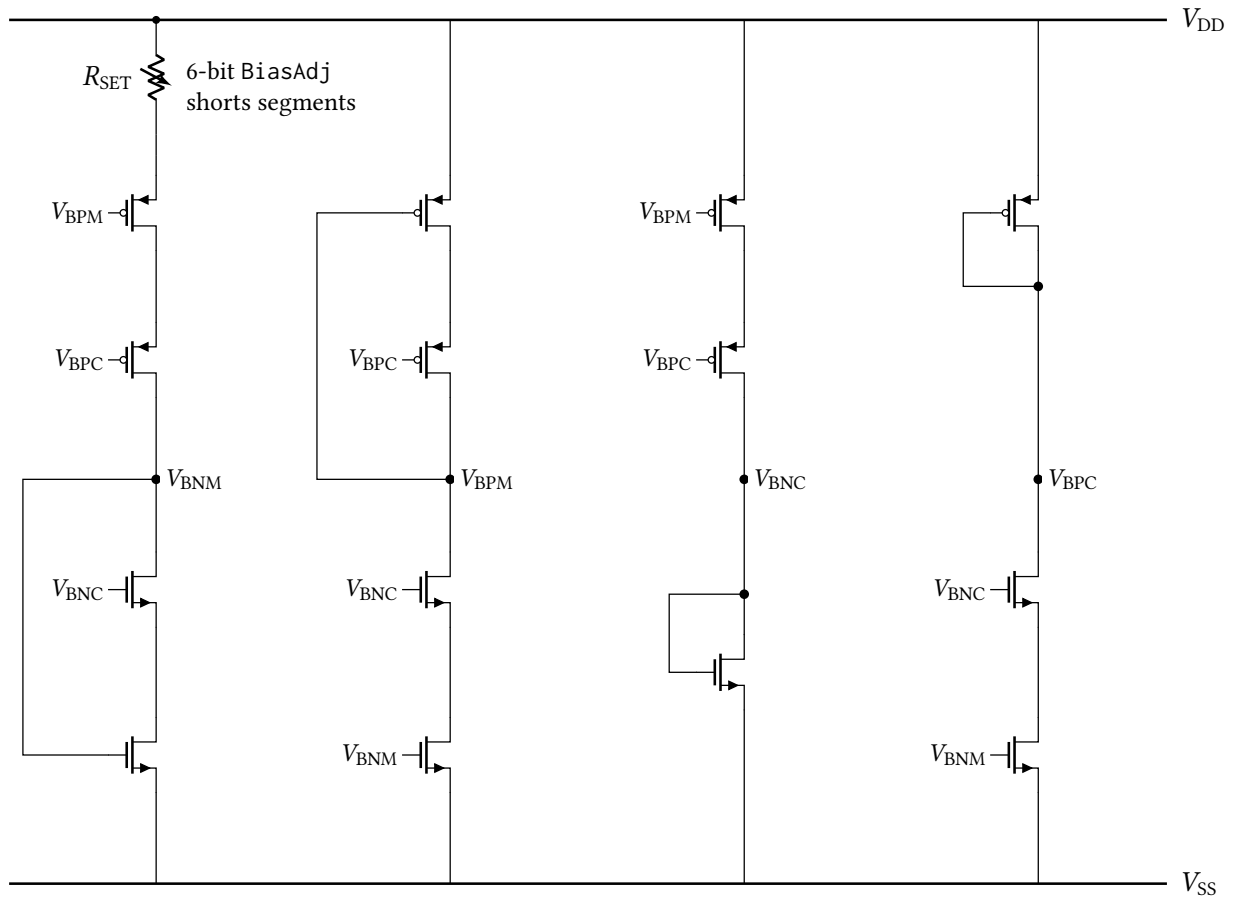
Figure 7: Simplified core of the local wide-swing cascode bias generator, drawn from the anatop_biasgen_local schematic. Four self-biased branches develop the four rails: the reference branch (left) passes the current set by the trimmable resistor R_{\text{SET}} , and the remaining branches mirror it to produce V_{\text{BPM}} , V_{\text{BNC}} and V_{\text{BPC}} . Each branch's own self-bias (diode) connection is drawn, from the rail it generates back to the gate it drives in the same branch; the cross-branch gate connections are identified by net name rather than drawn as buses. The enable switches, the decoupling capacitors on each rail and the individual segments of the resistor string are omitted for clarity.
