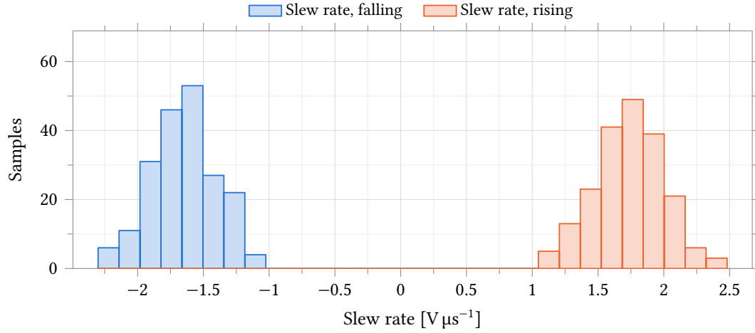
Figure 25: Slew rate on both edges of a 1 V step into 10 pF. Rising and falling averages are 1.74 \text{ V } \mu\text{s}^{-1} and 1.65 \text{ V } \mu\text{s}^{-1} , a 5 % imbalance: the tail current is steered into one input device and mirrored to the output, so the slewing current is equal in both directions by construction.
