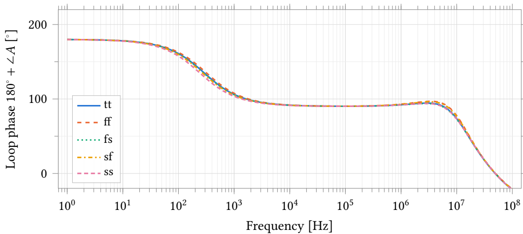
Figure 29: Phase of the same measurement. Spectre's stb reports 180^\circ + \angle A , so the value at crossover is the phase margin. The lift from 90.3^\circ at 100 kHz to 92.3^\circ at 1 MHz is the left-half-plane zero of Equation (4) adding lead, which holds the margin near 88^\circ through crossover despite the second pole at 10.8 MHz.
