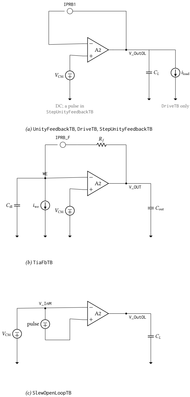
Figure 27: Testbenches for the transimpedance stage, from their netlists. (a) Unity feedback through a current probe with C_L = 5 pF: stb gives loop gain and phase, adding a swept i_{load} makes DriveTB, and a pulsed source StepUnityFeedbackTB. (b) The closed transimpedance loop; the electrode is a bare 1 \mu\text{F} to ground, not the Randles cell of Figure 6 — the caveat of Section 5.4.3. (c) Open-loop differential pulse drive. Supplies, bias trim buses and the enable pin are omitted throughout.
