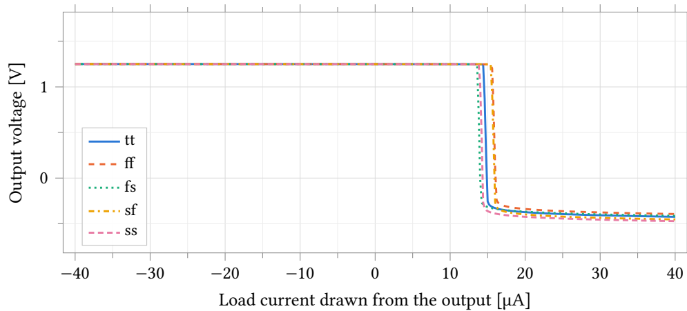
Figure 30: Output voltage as a DC load current is drawn from the output, over the five corners. Positive current is drawn out of the node, so the amplifier must source it; the collapse at 13.6\ \mu\text{A} to 15.6\ \mu\text{A} is the class-A stage running out of the fixed current in M5. Sinking holds within 0.8\ \text{mV} of v_{cm} to the -40\ \mu\text{A} sweep limit, so that direction is bounded, not measured.
